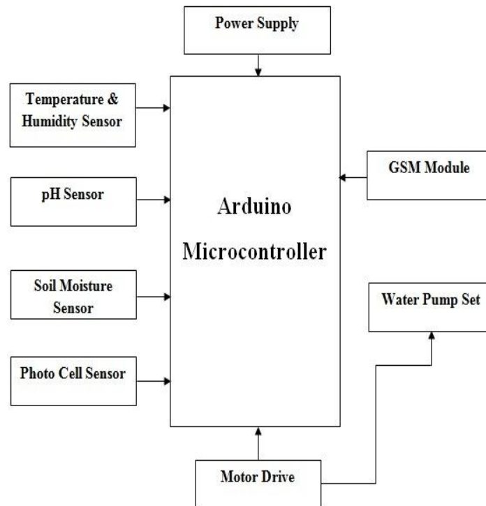
Fig.8: Block diagram of Smart irrigation System
