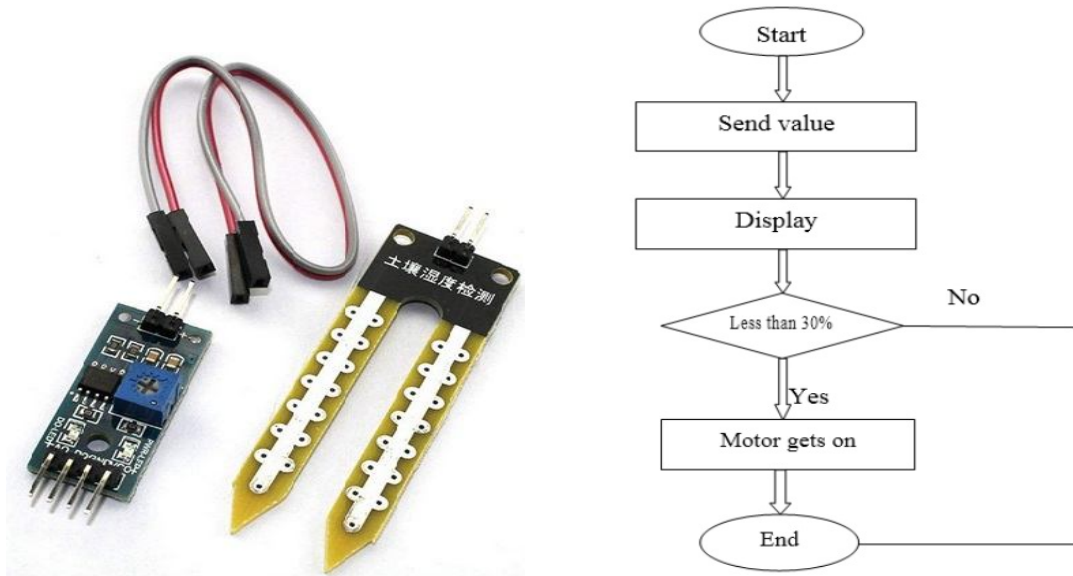
Fig.5: Soil Moisture Sensor and working Flow Chart[13]
