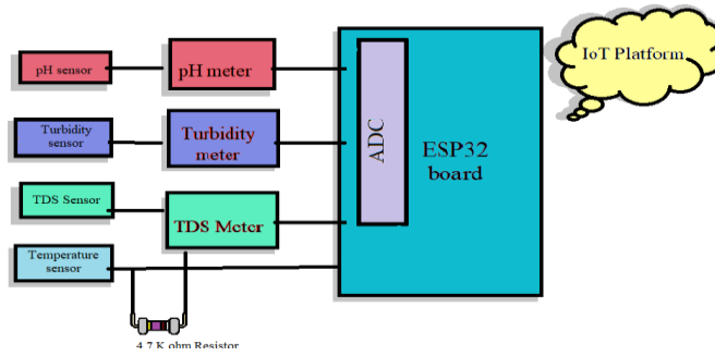
Fig.3. Block diagram
