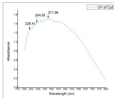
Figure 1: Ultraviolet visible Spectrum of CuO
