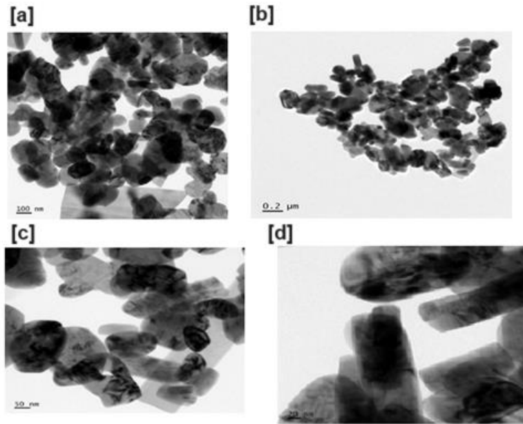
Figure 5: Transmission Electron Microscopy Images of [a] 100nm, [b] 0.2µm, [c] 50nm and [d] 20nm
