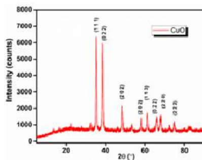
Figure 2a: X-ray Diffraction of CuO
