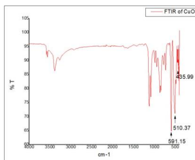
Figure 3: Fourier transform infrared of CuO
