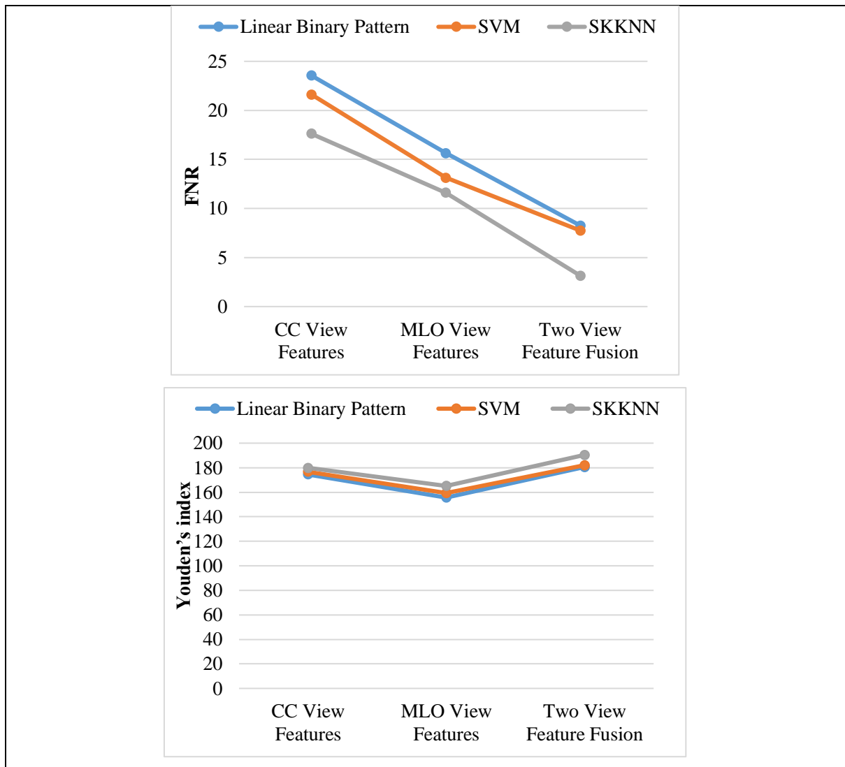
Figure 3.1 Chart Comparison of Linear Binary Pattern, SVM and SKKNN
