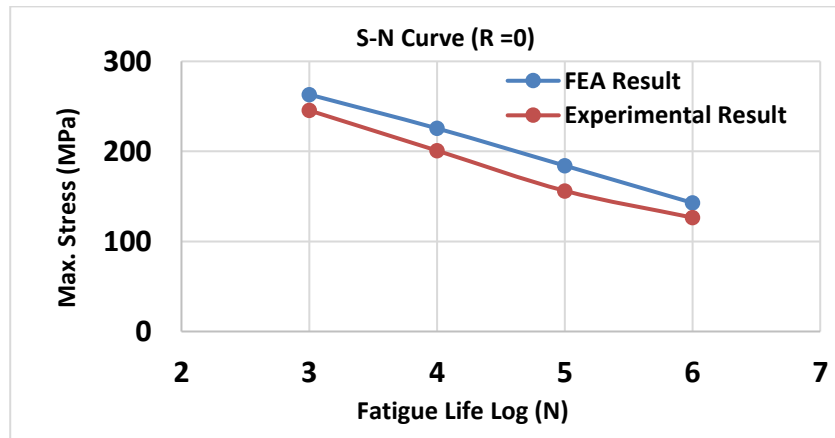
Figure 19: Fatigue Life of [45/90/-45/0] s Laminates
