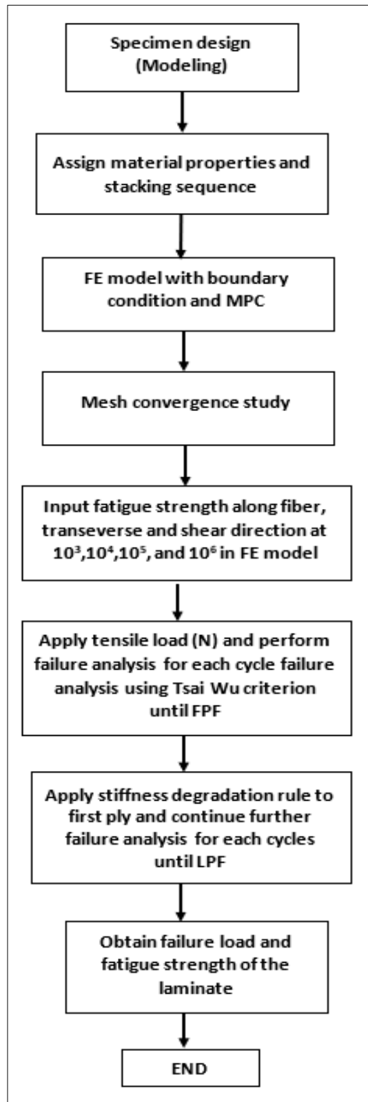
Figure 13: Flow Chart for Fatigue Analysis
