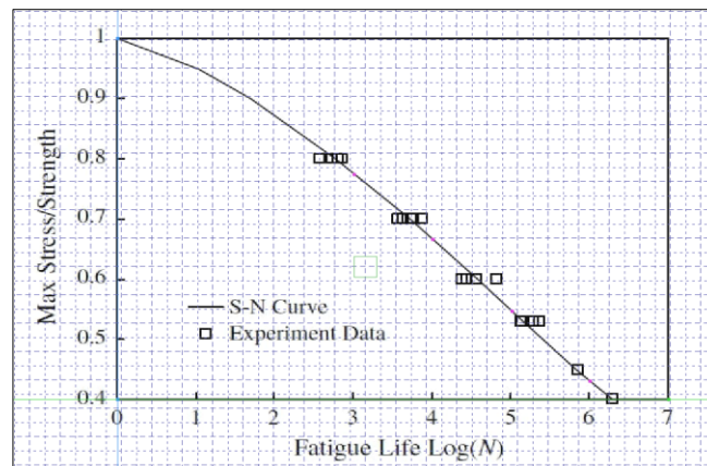
Figure 2: Standard S-N Curve of [0]_8 Laminates [1]
