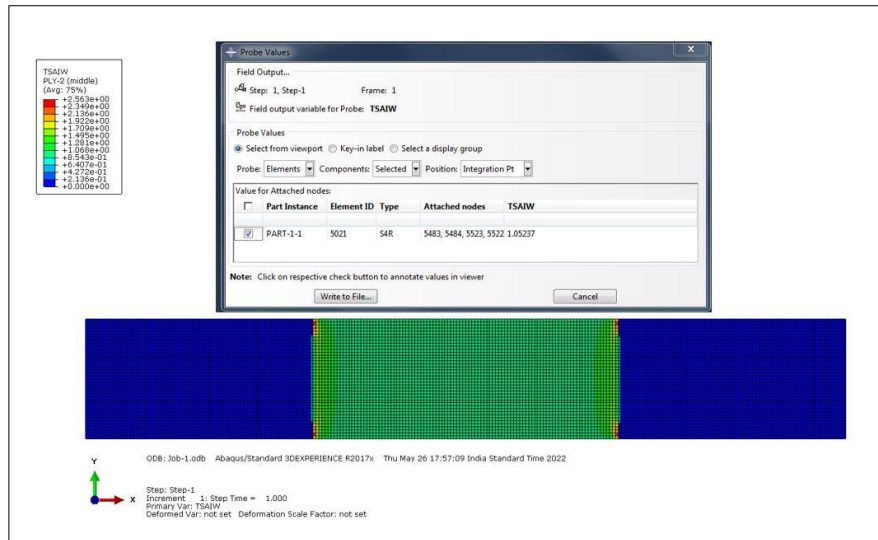
Figure 17: Failure Index Value of 0° Last Ply Failure using Tsai Wu Rule
