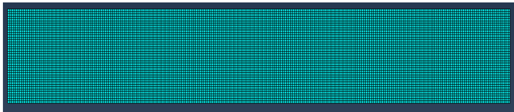
Figure 8: FE Mesh of Unnotched Composite Laminate
