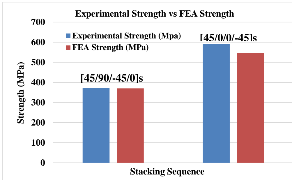
Figure 18: Error Bar Comparison of Experimental Strength [1] vs FEA Strength
