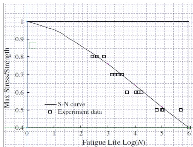
Figure 3: Standard S-N Curve of [90]_8 Laminates [1]
