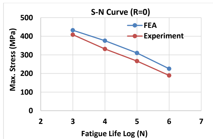
Figure 21: Fatigue Life of [45/0/0/-45]s Laminates
