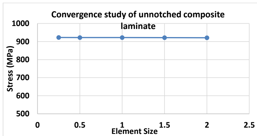
Figure 9: Variation of Stress With Different Element Sizes
