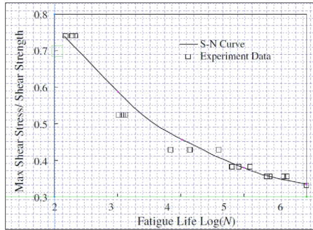
Figure 4: Standard S-N Curve Under in-plane Shear Stress [1]
