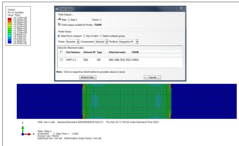
Figure 22: Failure Index Value of 0° Last Ply Failure at 10 6 Cycle using Tsai Wu criterion
