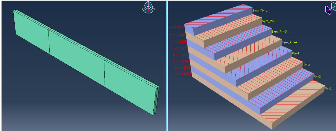
Figure 7: Stacking Plot [45/0/0-45]s
