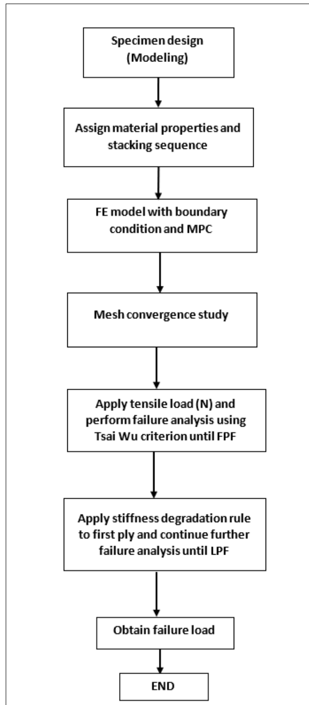
Figure 12: Flow Chart for Static Analysis
