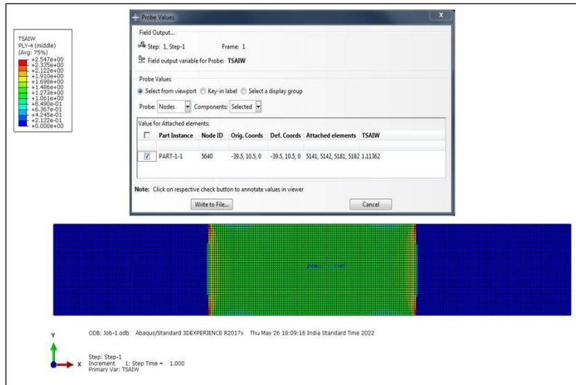
Figure 15: Failure Index Value of 0° Last Ply Failure using Tsai Wu Rule
