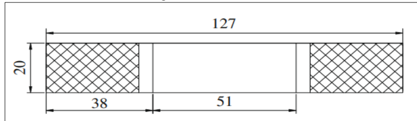
Figure 1: Specimen Geometry (mm)
