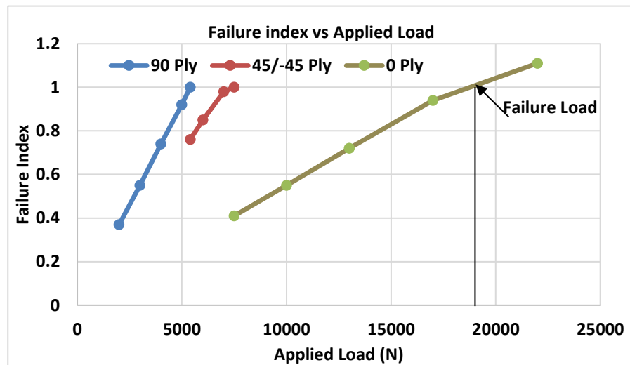
Figure 14: Failure Index vs Applied Load (N) of [45/90/-45/0]s laminate
