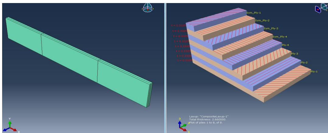
Figure 6: Stacking Plot [45/90/-45/0] s
