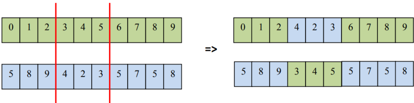
Fig 8. Multipoint crossover
