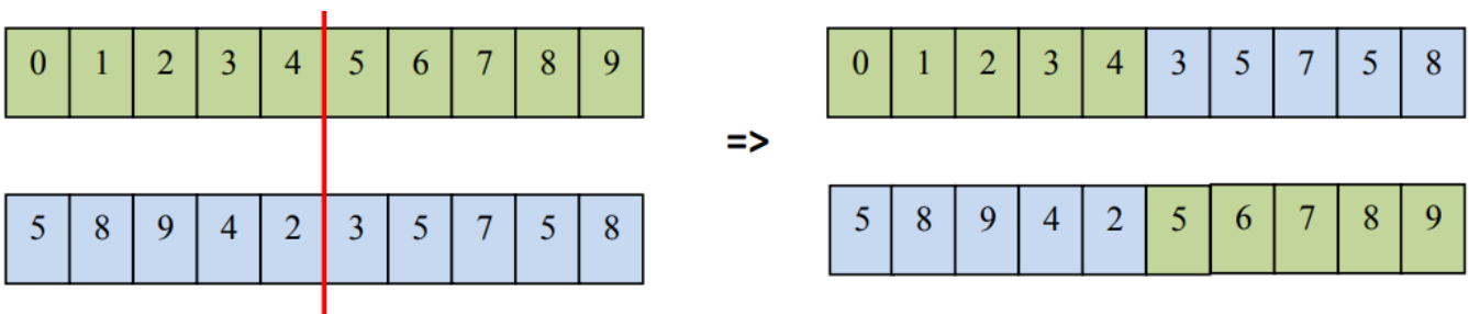
Fig.7.One-Point-CrossOver
