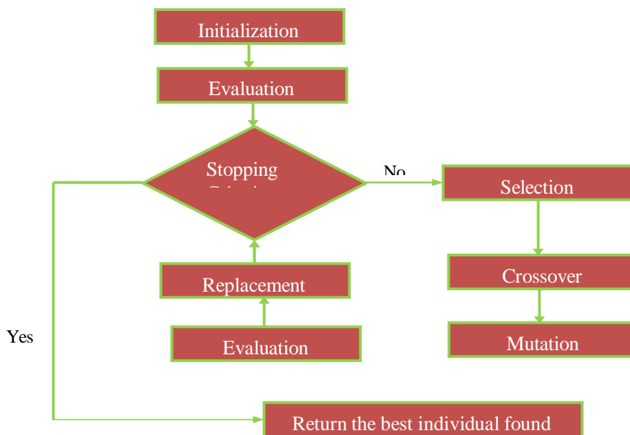
Fig 5. GA Cycle
