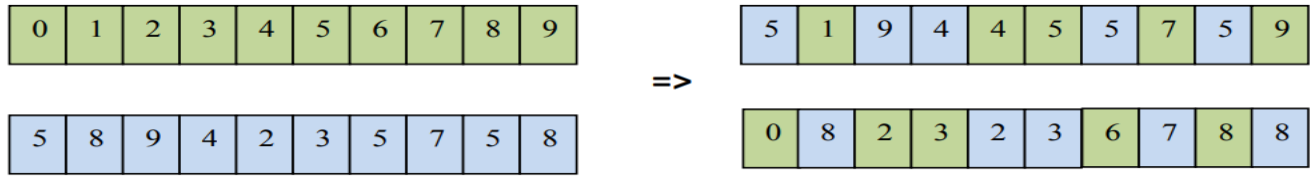
Fig 9. Uniform crossover
