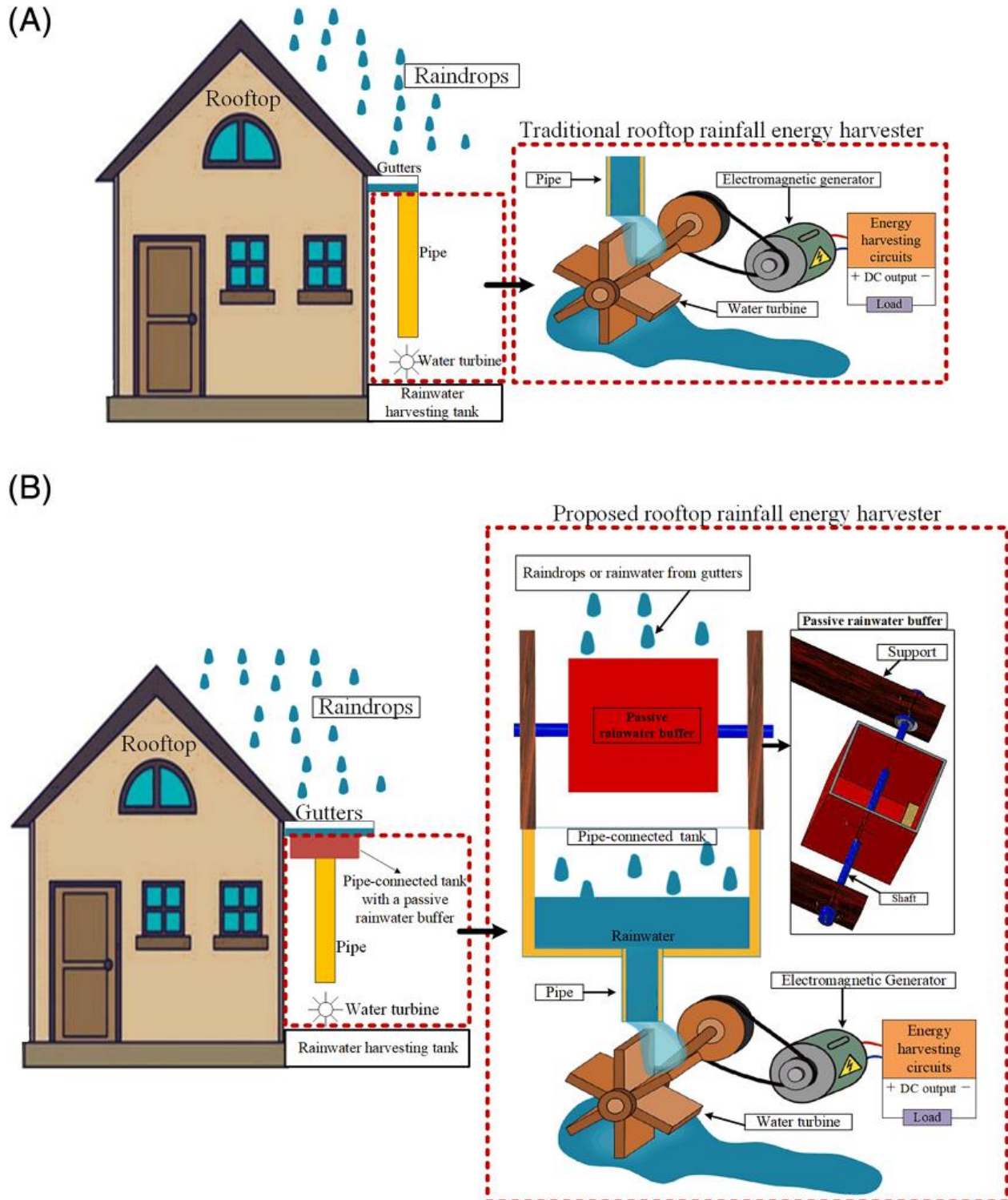
Fig. 3. Rains water electric power generation system.
