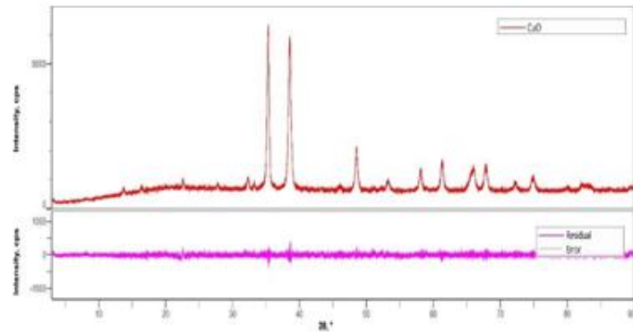
Fig 3: Peak Profile of CuO
