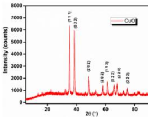
Fig 2: X-ray Diffraction of CuO
