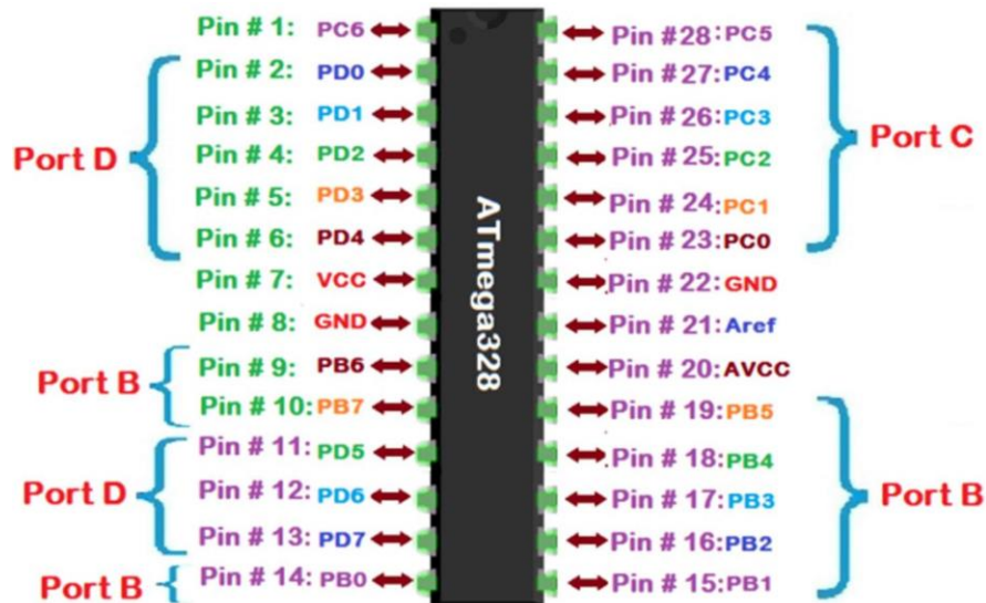
Fig 5.6 Pin diagram
