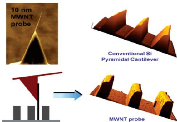
Figure 7. Comparison of the AFM depictions captured from the multiwalled CNT probe and the silicon probe. (Valcárcel et al., 2007) Reprinted with permission from Valcárcel, M., Cárdenas, S. & Simonet, B. M. Role of Carbon Nanotubes in Analytical Science. Anal. Chem. 79, 4788–4797 (2007). Copyright
