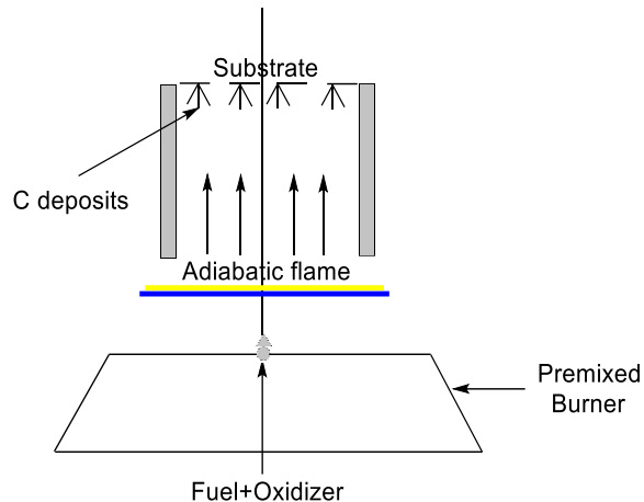
Figure 4. Schematic representation of hydrocarbon flames method for synthesis of CNTs
