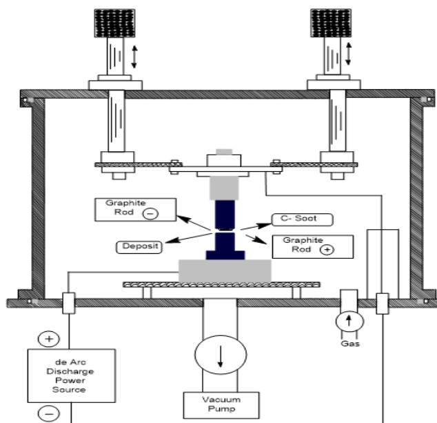
Figure 1. Arc evaporation apparatus for producing CNTs
