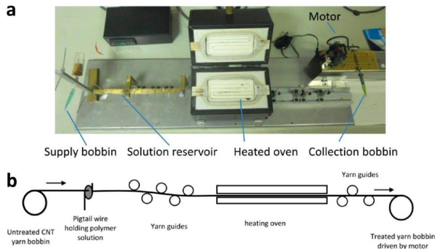
Figure 12. (a) Image, and (b) graphic of the continual dip-coating line utilized for the solution polyaniline nanowire and the gel PVA-H 3 PO 4 .(Su et al., 2014) Reprinted with permission from Su, F., Miao, M., Niu, H. & Wei, Z. Gamma-Irradiated Carbon Nanotube Yarn As Substrate for High-Performance Fiber Supercapacitors. ACS Appl. Mater. Interfaces 6, 2553–2560 (2014). Copyright (2014) American Chemical Society.
