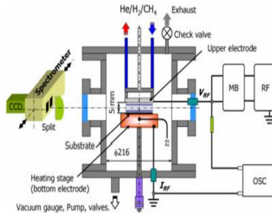
Figure 3. Measurement system and reactor of APRFD. Reprinted with permission from Nozaki, T., Ohnishi, K., Okazaki, K. & Kortshagen, U. Fabrication of vertically aligned single-walled carbon nanotubes in atmospheric pressure non-thermal plasma CVD. Carbon N. Y. 45, 364–374 (2007). Copyright (2007) Elsevier Ltd.
