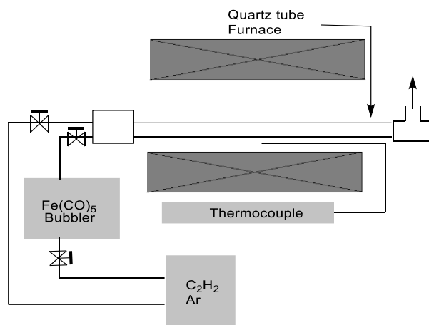
Figure 5. Schematic diagram for the vapor phase growth system.
