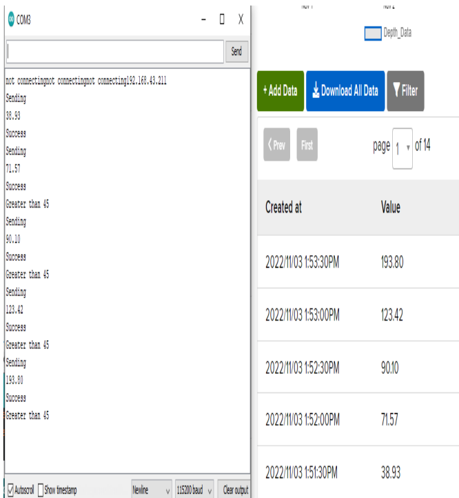
Figure 6. Fuel level in Serial monitor and adafruit cloud
