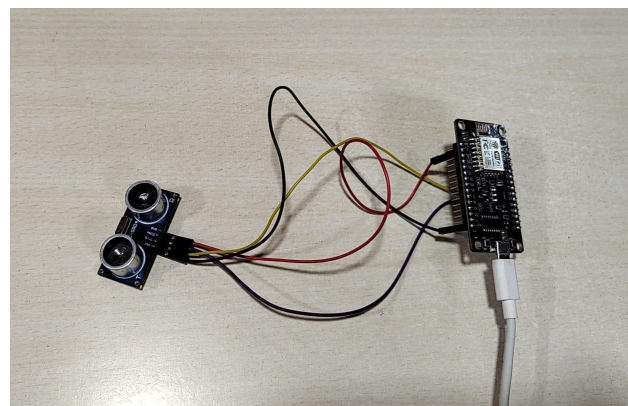
Figure 4: Connection of NodeMCU with ultrasonic sound sensor
