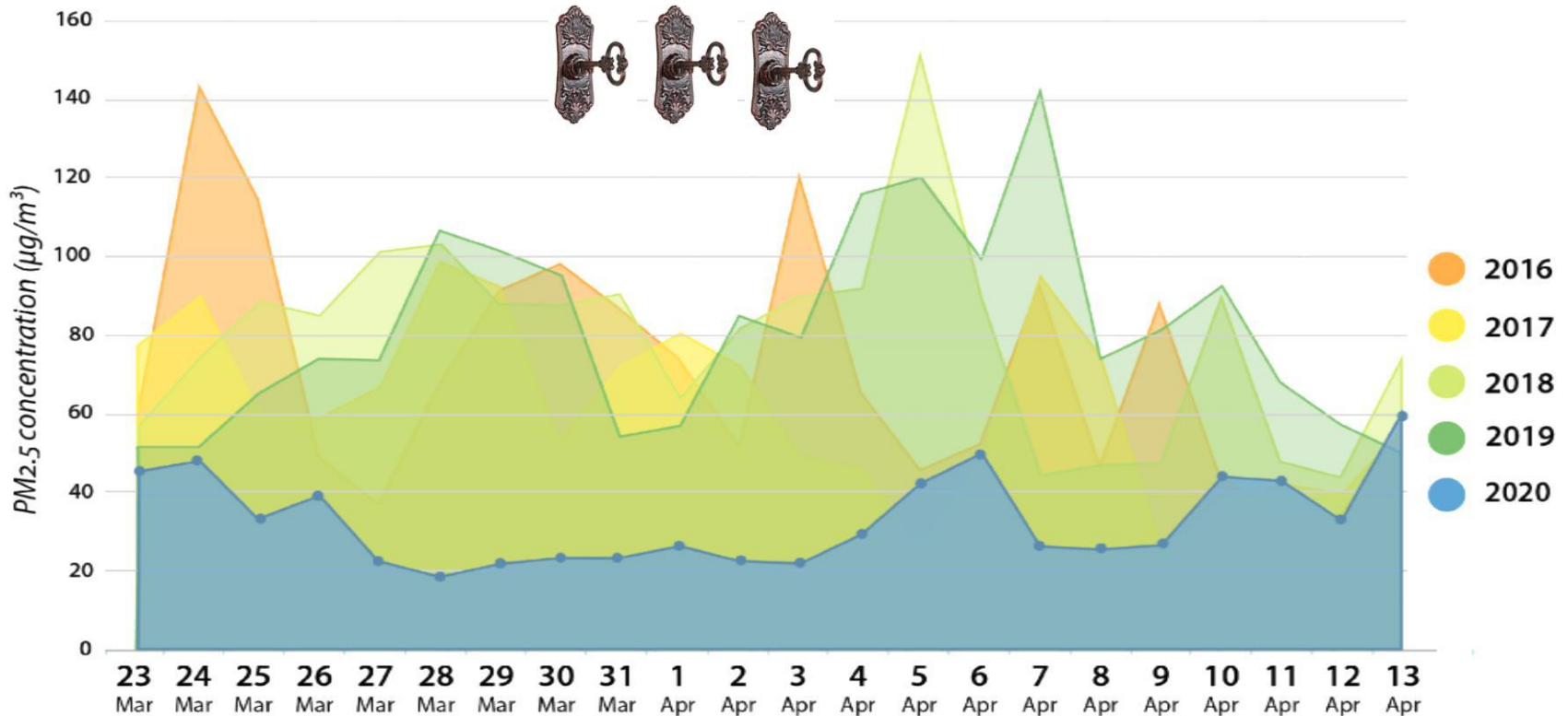
Daily PM2.5 levels in Delhi, India from 2016-2020, during the 2020 lockdown period 23 March - 13 April
