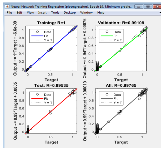
Figure (5.7) Regression curve.
