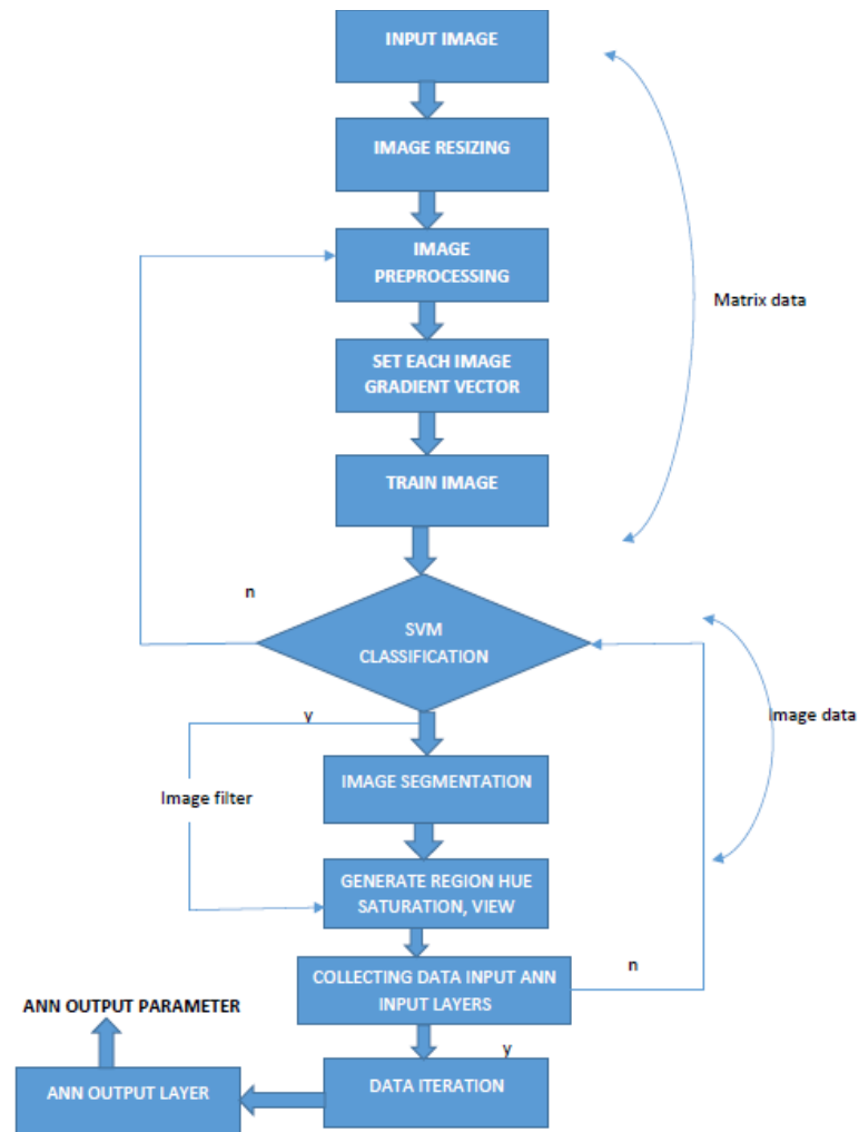
Figure (4.6) Flow chart proposed algorithm.
