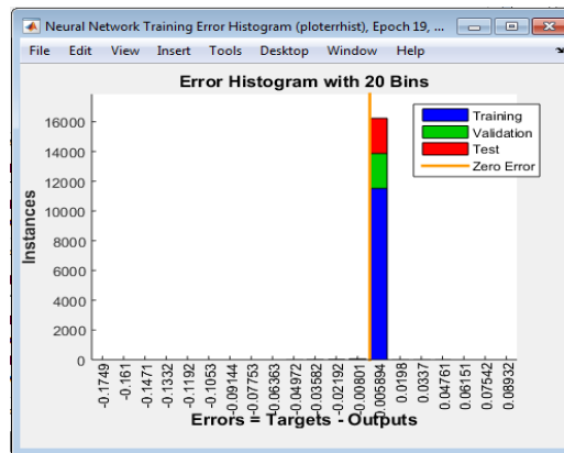
Figure (5.6) Error variation across on train, validation and test.
