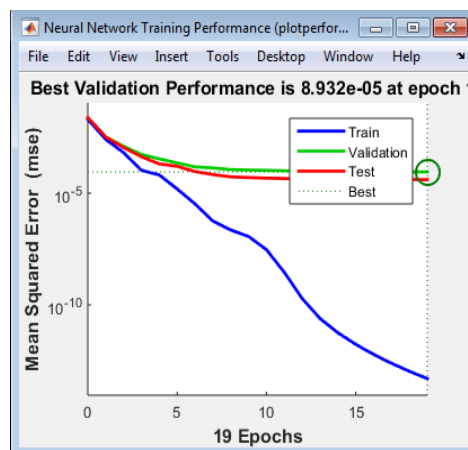
Figure (5.5) MSE criteria based performance evaluation.
