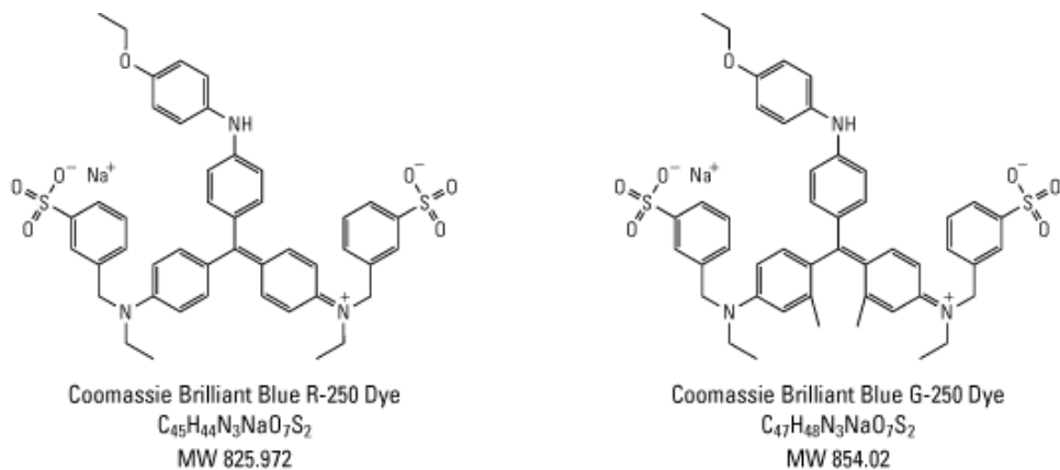
Figure 8: -The structure of Coomassie brilliant blue [8,9].
