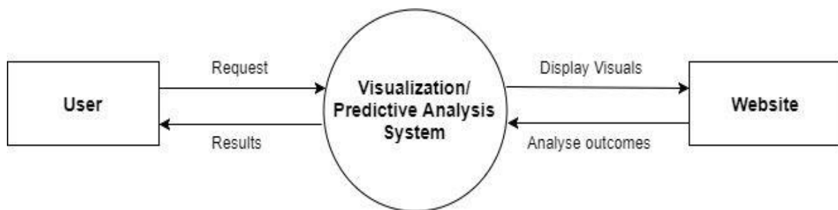
Figure 1. Architectural DFD
