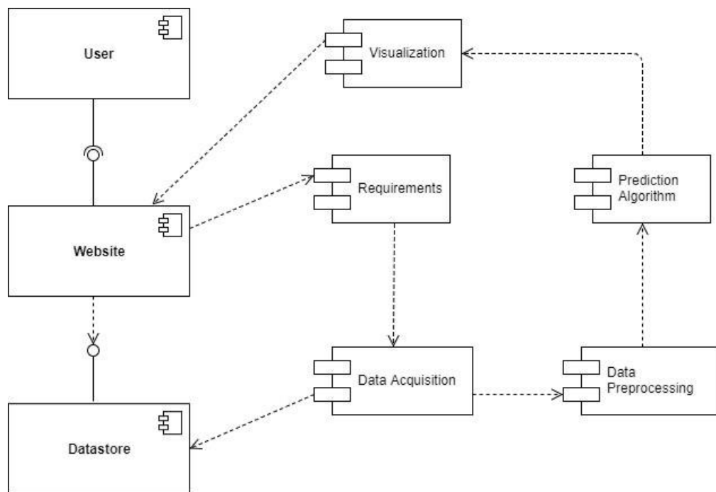
Figure 3: Component Diagram
