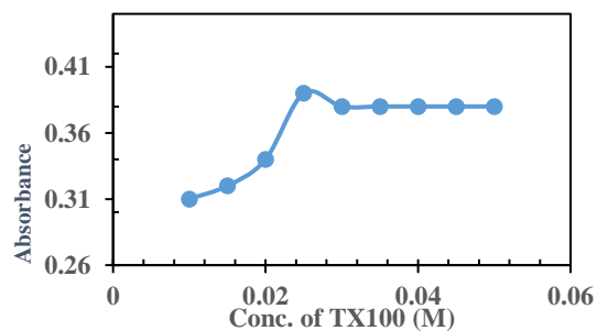
Fig.2. The influence of Triton X-100 concentration on the absorbance of 0.5 \mu\text{g ml}^{-1} of BG after cloud point extraction at pH 3.5.
