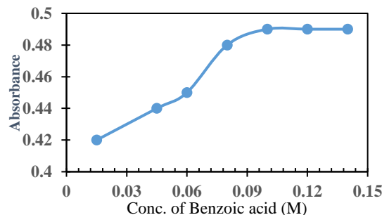
Fig.3. The effect of benzoic acid concentration on the absorption of 0.5 \mu\text{g ml}^{-1} of BG after cloud point extraction at pH 3.5 and 0.025 \text{ mol L}^{-1} Triton X-100.
