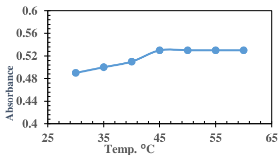
Fig.4. The effect of temperature on the absorption of 0.5 \mu\text{g ml}^{-1} of BG after cloud point extraction at pH 3.5, 0.025 \text{ mol L}^{-1} Triton X-100 and 0.1 \text{ mol L}^{-1} benzoic acid.
