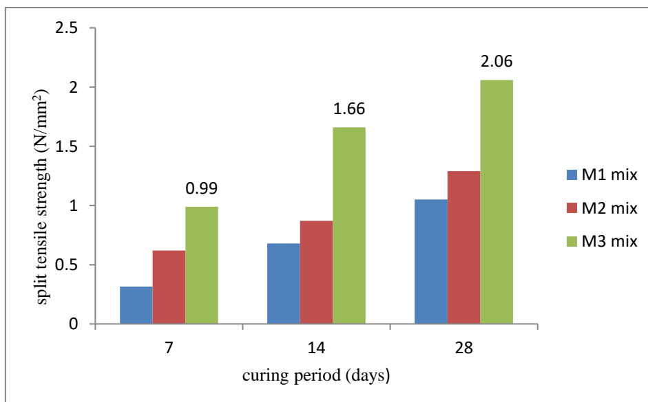
Figure 3. Effect of curing period on split tensile strength.
