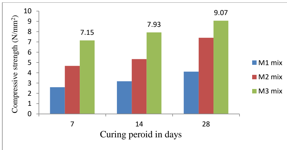
Figure 2. Effect of curing period on compressive strength
