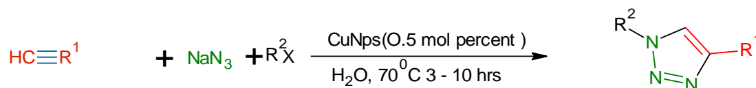
Scheme 14 : Synthesis of substituted triazoles using Cu NPs
