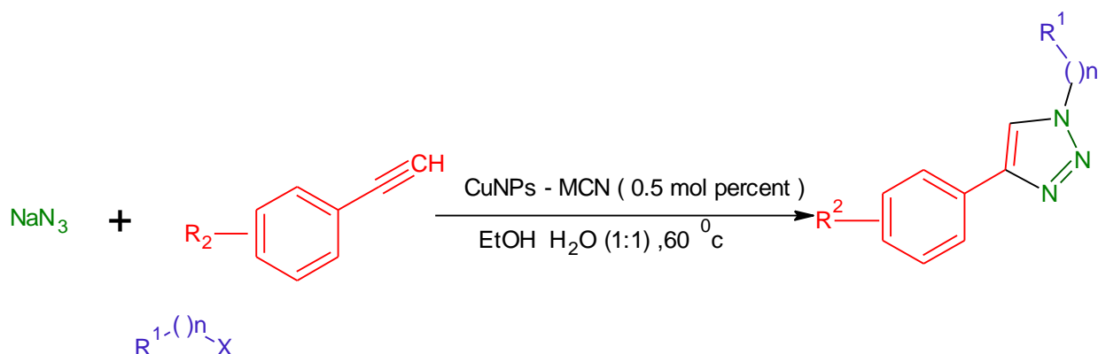
Scheme 20: Cu NP-catalyzed 1,3-dipolar cycloaddition for the synthesis of triazoles
