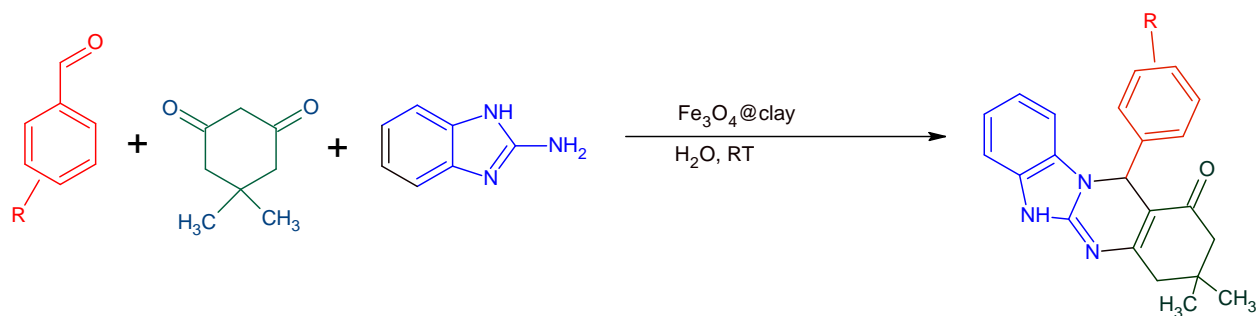
Scheme 36: Ultrasonic-assisted synthesis of imidazo(thiazolo)pyrimidines by using Fe_3O_4@clay nanocatalyst
