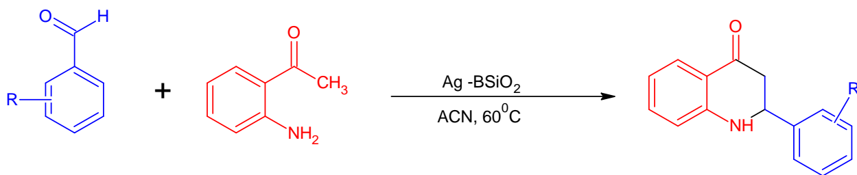
Scheme 30: Synthesis of dihydroquinoline.
