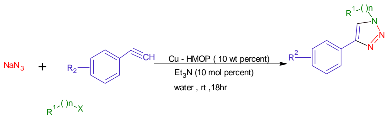
Scheme 19: Click reaction for the synthesis of triazoles catalyzed by Cu-HMOP.
