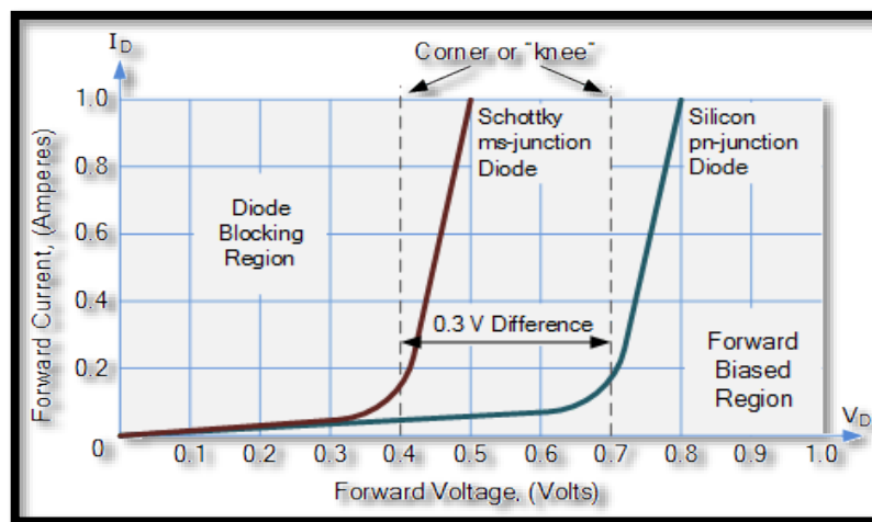
Fig. 20. Schottky Diode V-I Characteristics
