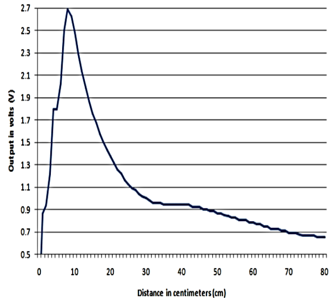
Fig 4.0 Distance Measurement with respect to voltage
