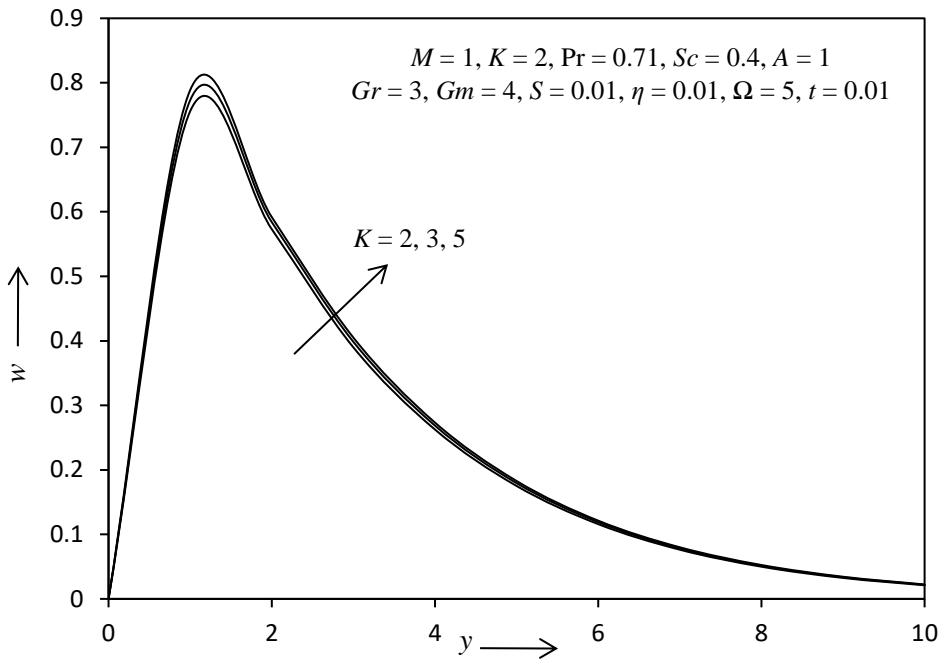
Fig. 6: The secondary velocity profile for different values of K .
