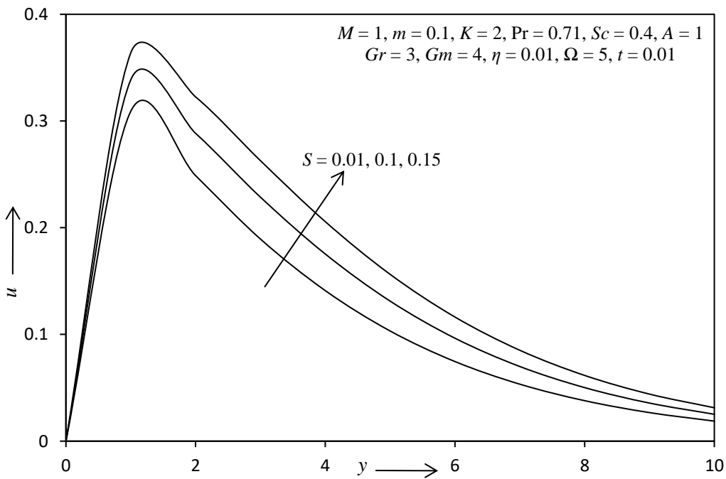
Fig. - 11: The primary velocity profile for different value of S .
