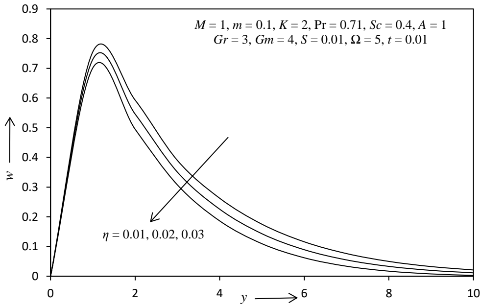
Fig. 22: The secondary velocity profile for different values of \eta .
