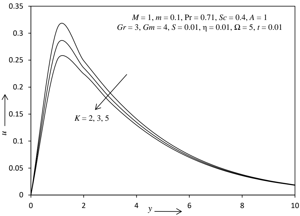
Fig. - 5: The primary velocity profile for different value of K .
