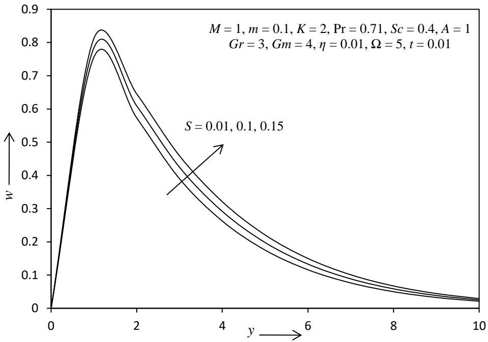
Fig. 18: The secondary velocity profile for different values of S .
