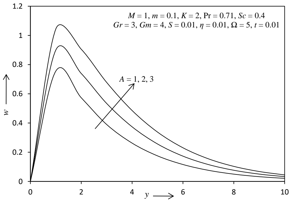
Fig. 17: The secondary velocity profile for different values of A .
