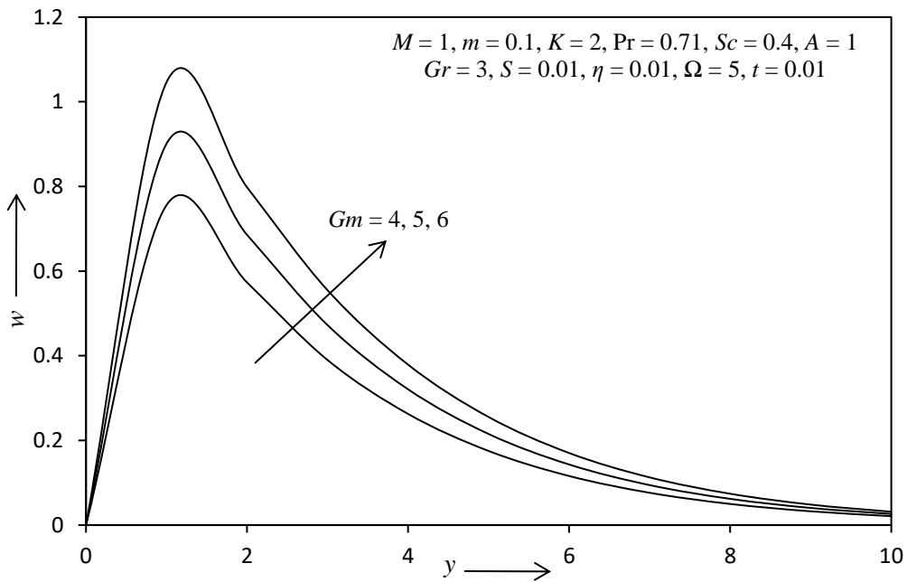
Fig. 15: The secondary velocity profile for different values of Gm .
