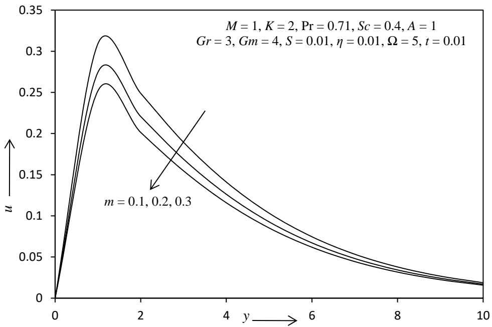
Fig. - 3: The primary velocity profile for different value of m .
