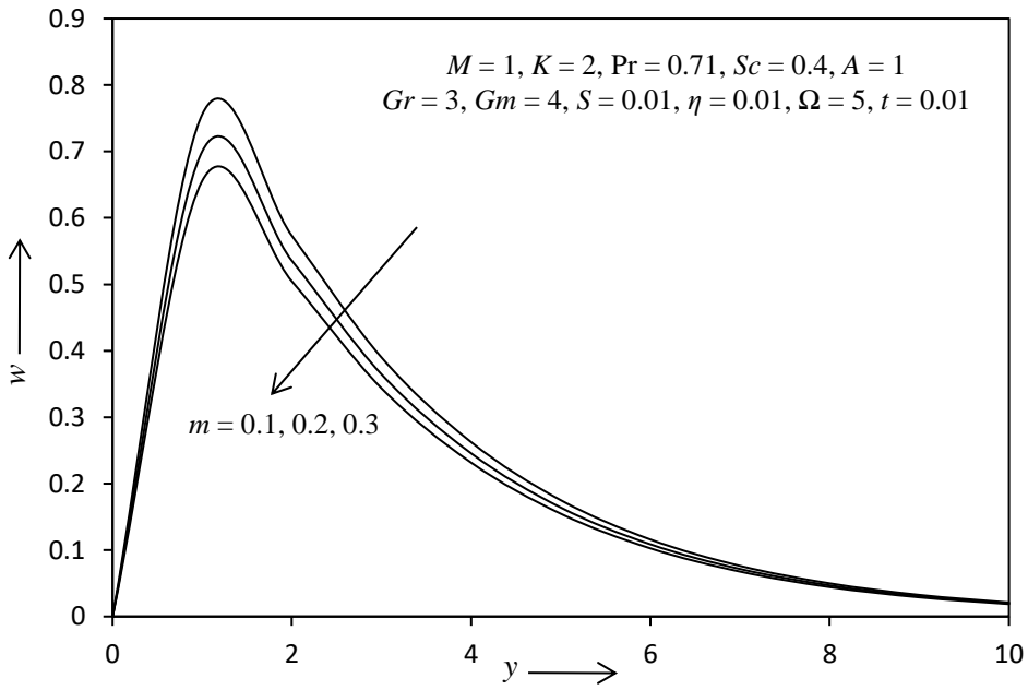
Fig. 4: The secondary velocity profile for different values of m .
