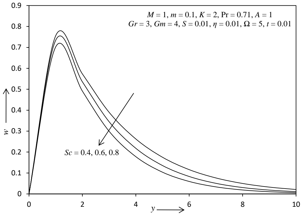
Fig. 20: The secondary velocity profile for different values of Sc .
