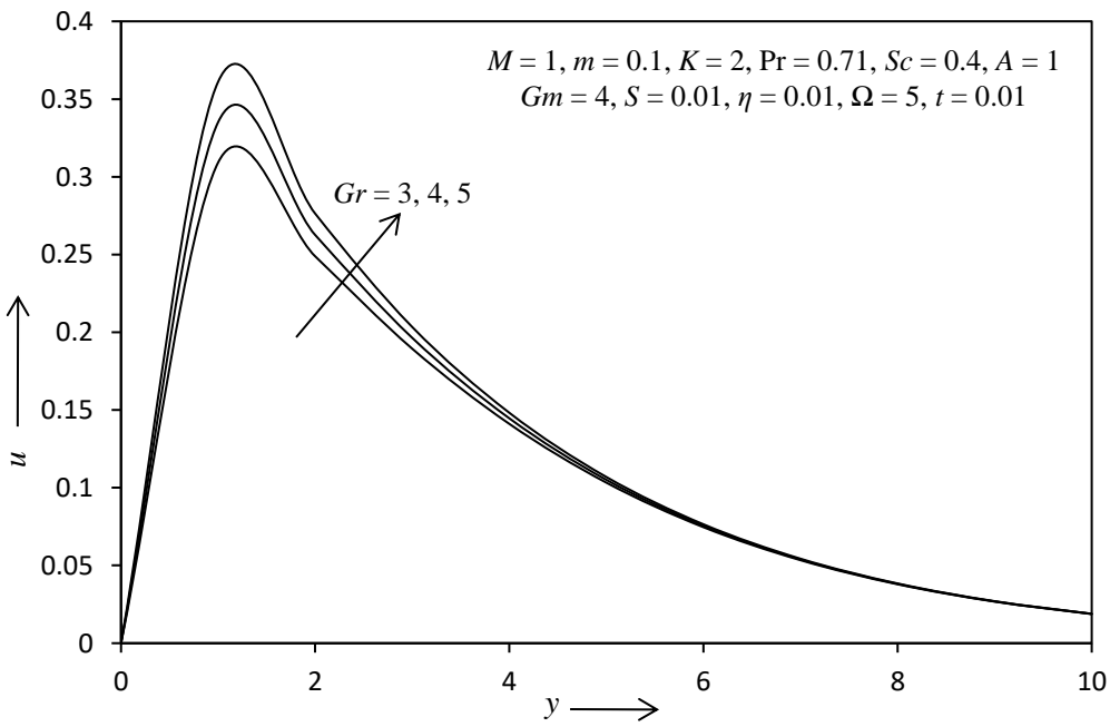
Fig. - 7: The primary velocity profile for different value of Gr .
