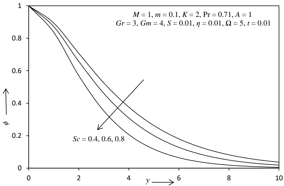
Fig. - 23: The Concentration Profile for different Value of Sc .
