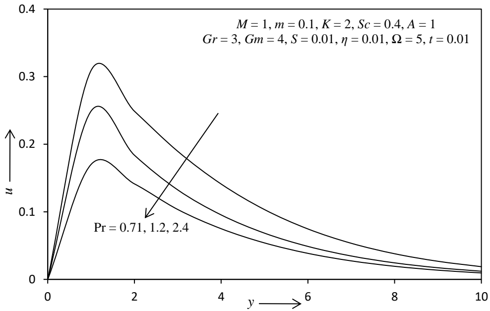
Fig. - 12: The primary velocity profile for different value of Pr.
