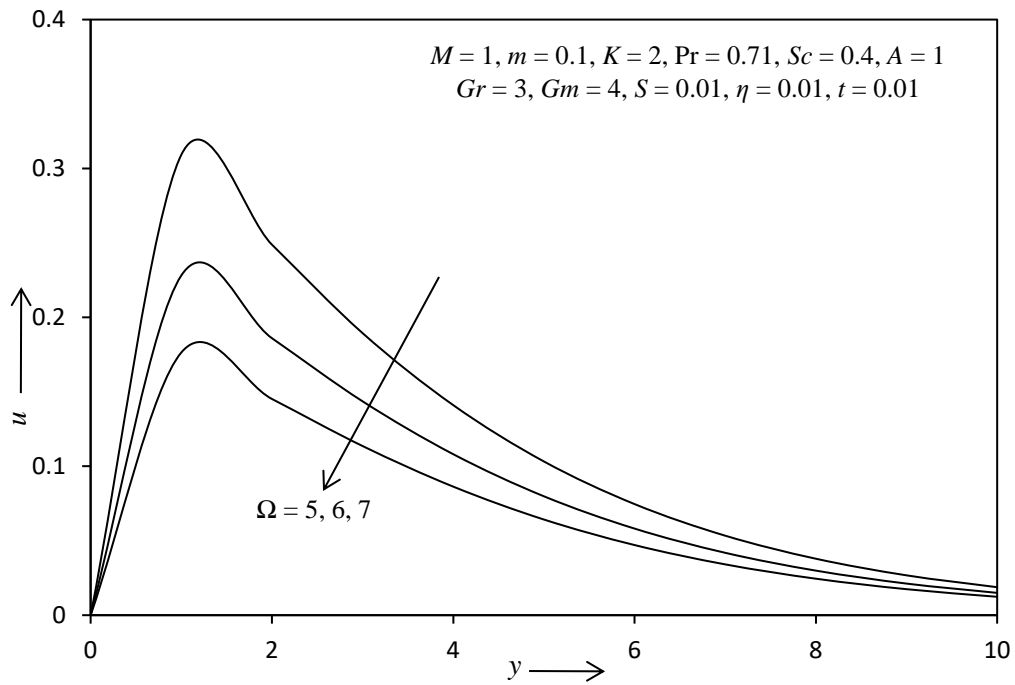
Fig. - 9: The primary velocity profile for different value of \Omega .
