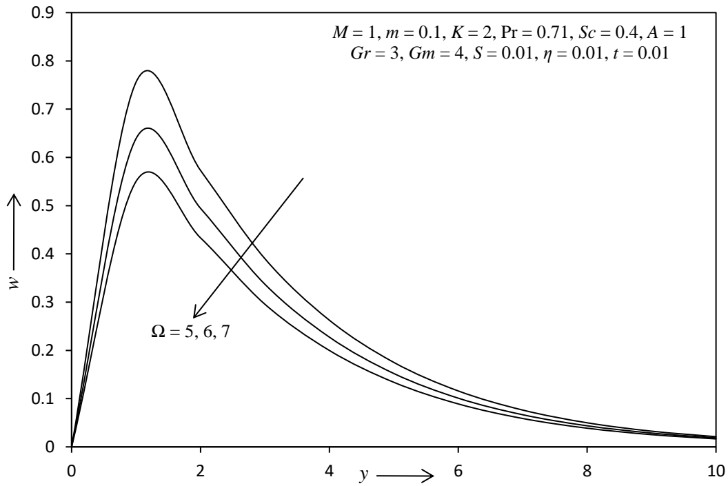
Fig. 16: The secondary velocity profile for different values of \Omega .
