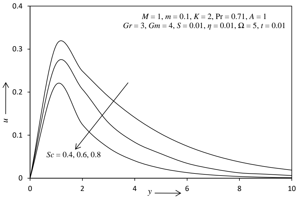
Fig. - 13: The primary velocity profile for different value of Sc.
