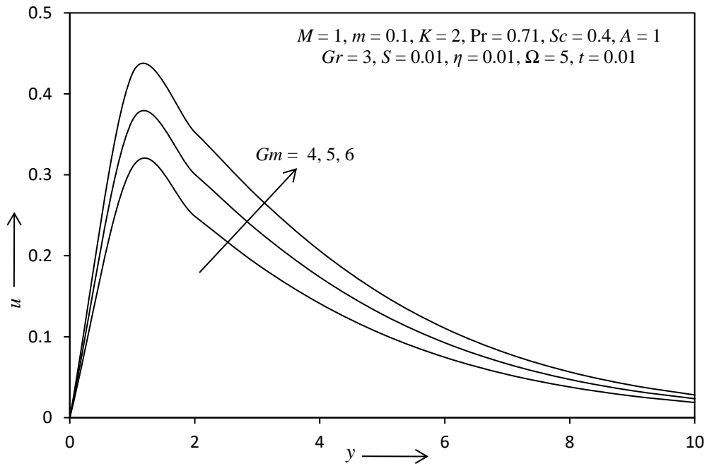
Fig. - 8: The primary velocity profile for different value of Gm .
