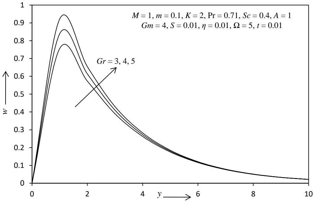
Fig. 14: The secondary velocity profile for different values of Gr .
