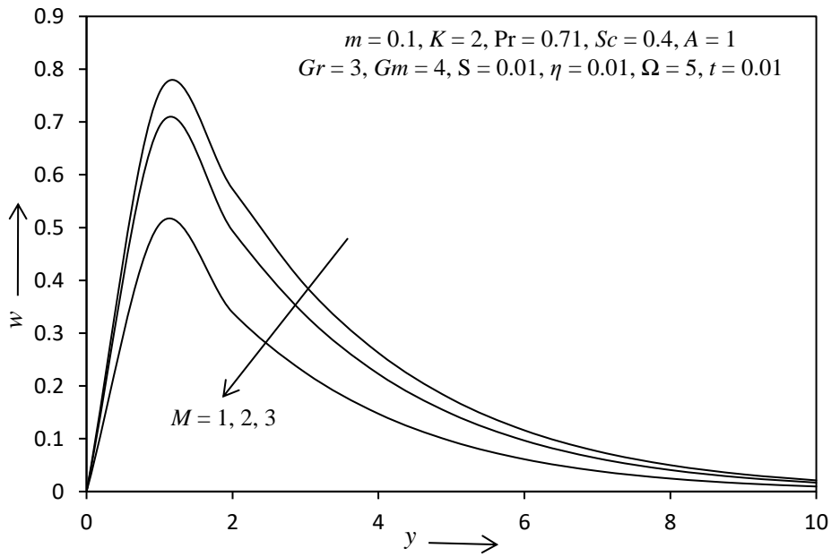
Fig. 2: The secondary velocity profile for different values of M .
