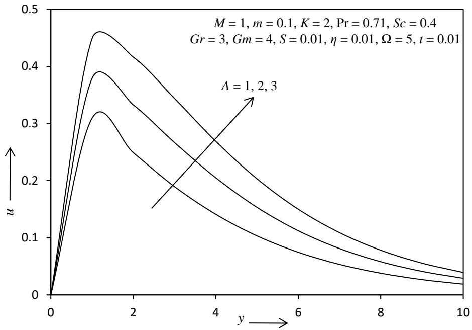
Fig. - 10: The primary velocity profile for different value of A .
