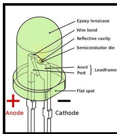
Fig. 16. LED Structure
