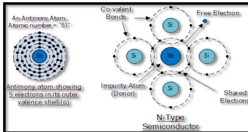
Fig.3. N – Type Extrinsic Semiconductor with Impurity Atoms
