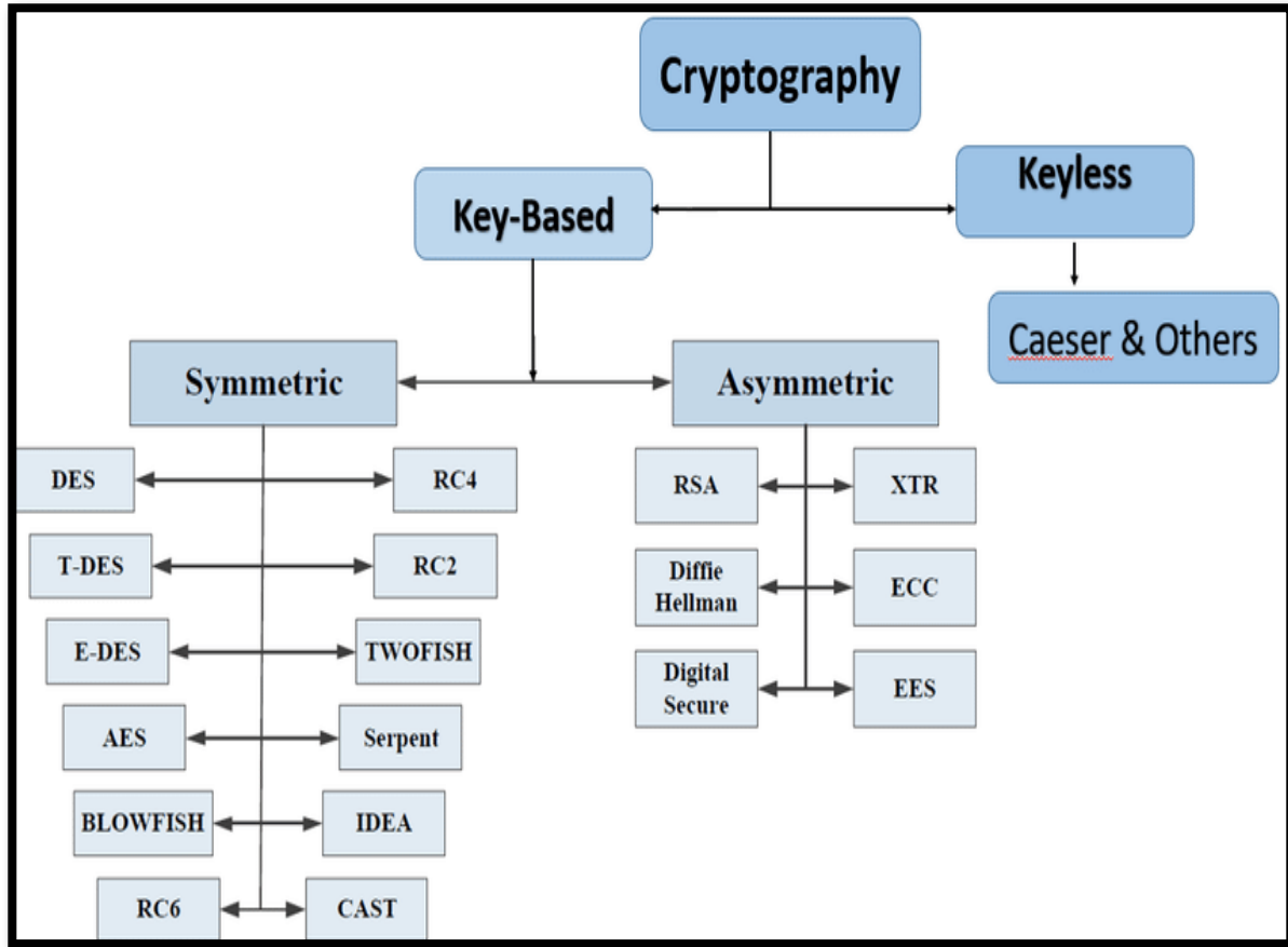
Figure 2: Different kinds of cryptographic currencies
