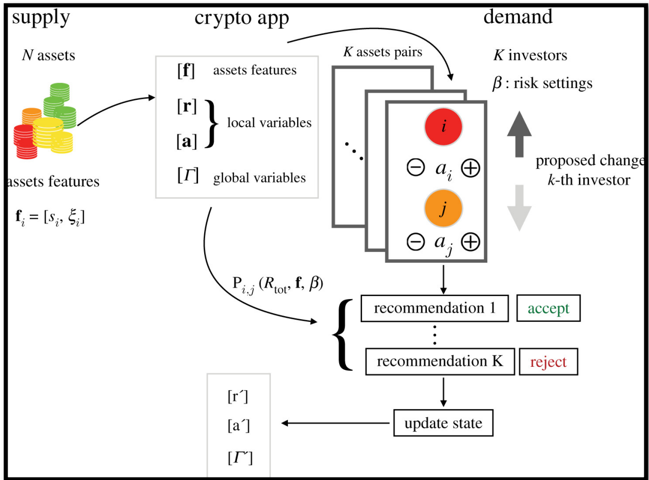
Figure 1: Cryptographic currencies
