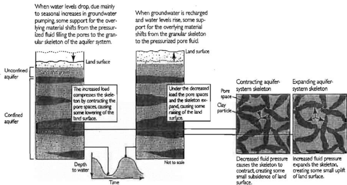
Figure 20. Relation between changes in groundwater level and compression of aquifer system (Galloway et al).
