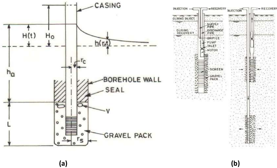
Figure 15 (a) Forced recharge and (b) Free recharge
