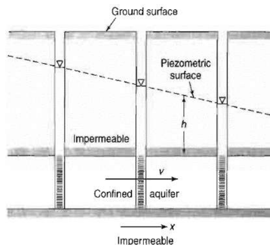
Figure 13 Steady unidirectional flow in a confined aquifer of uniform thickness.
