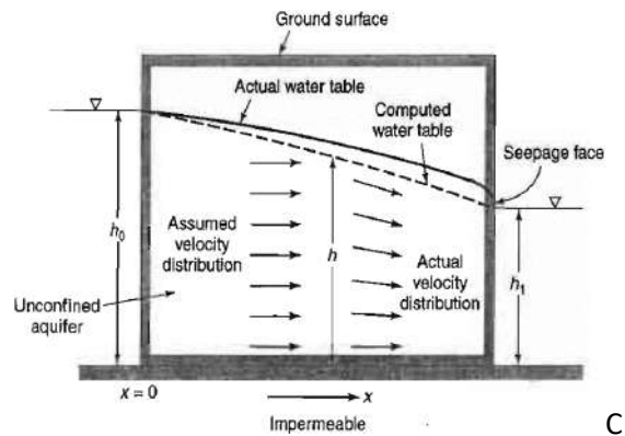
Figure 12. Steady flow in an unconfined aquifer between two water bodies with vertical boundaries.
