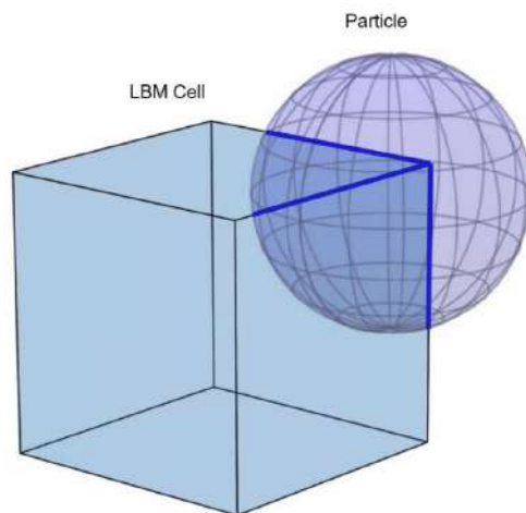
Figure 11 Schematic of Volume fraction when the DEM sphere particle interacts with LBM cell.
