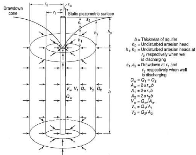
Figure 14 Radial flow from a fully penetrating well in a confined aquifer.
