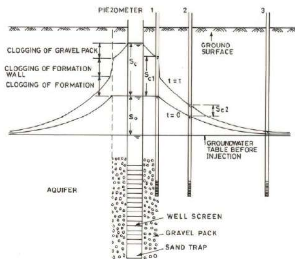
Figure 16 Well losses during well recharge
