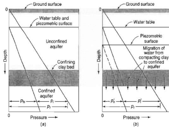
Figure 21 Graph of hydraulic and intergranular pressures as a function of depth for an unconfined aquifer overlying a confined aquifer (after Poland et al.). (a) Initial condition with water table and piezometric surface at same elevation (b) Subsequent condition with piezometric surface lowered.
