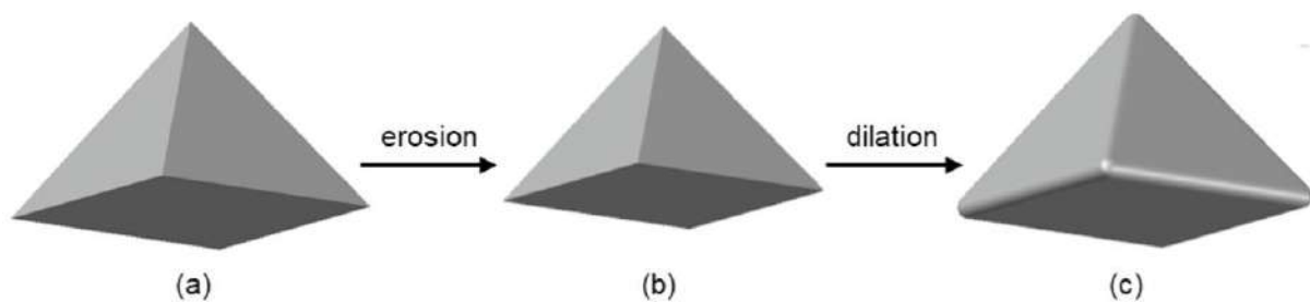
Figure 9 Particle construction in sphero-polyhedra based DEM (a) original geometry; (b) geometry after erosion; (c) geometry after dilation.
