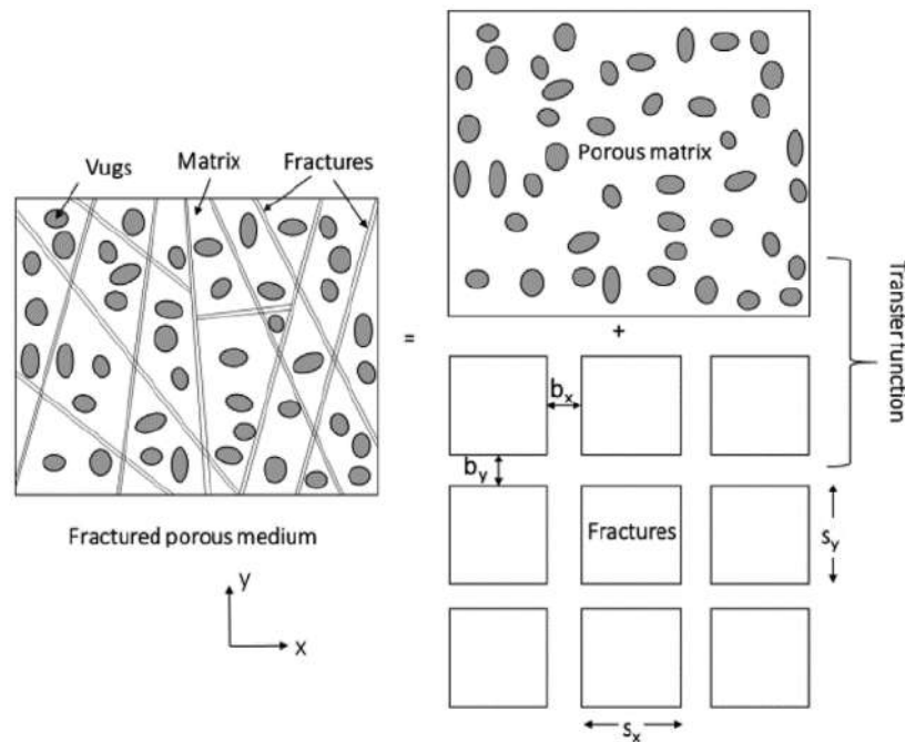
Figure 22. Idealization of naturally fractured system with dual porosity model.
