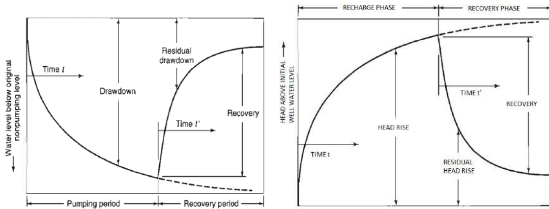
Figure 18. (a) Drawdown and recovery curves, (b) Recharge and Recovery curves.
