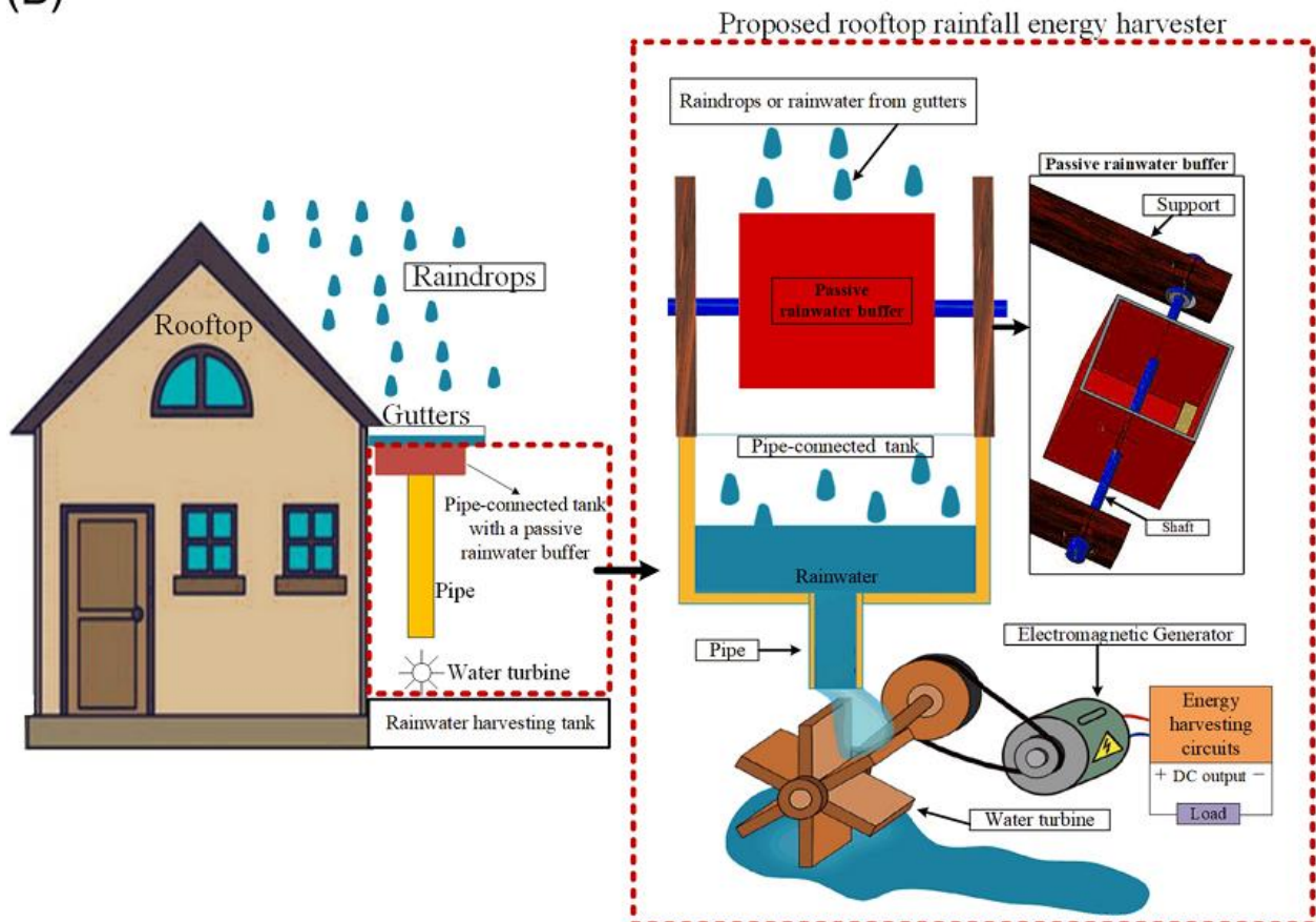
Fig. 3. Rains water electric power generation system.
