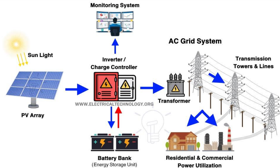
Fig. 2. Solar electric power plant system.
