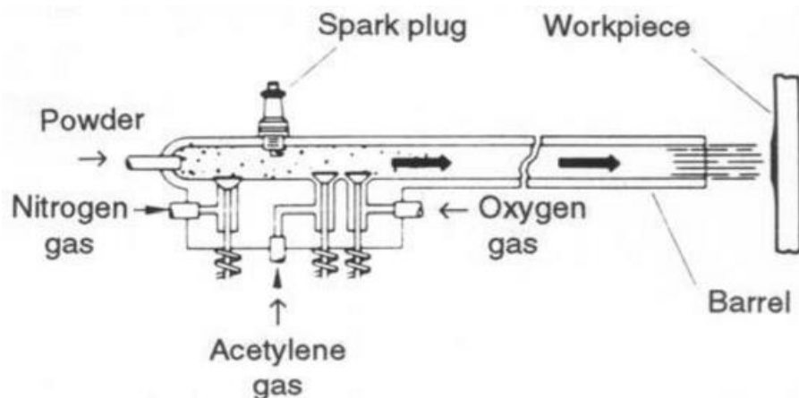
Fig 6: D-Gun [35]
