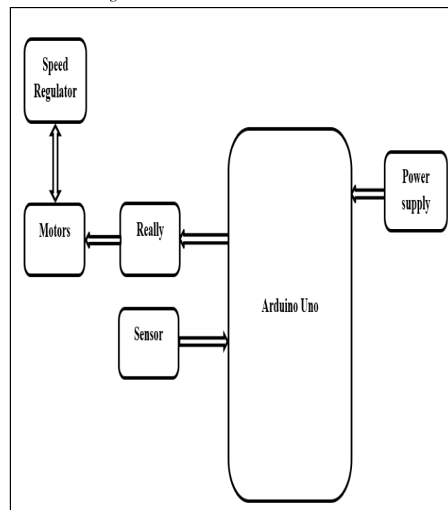
Fig 4.1: Block Diagram
