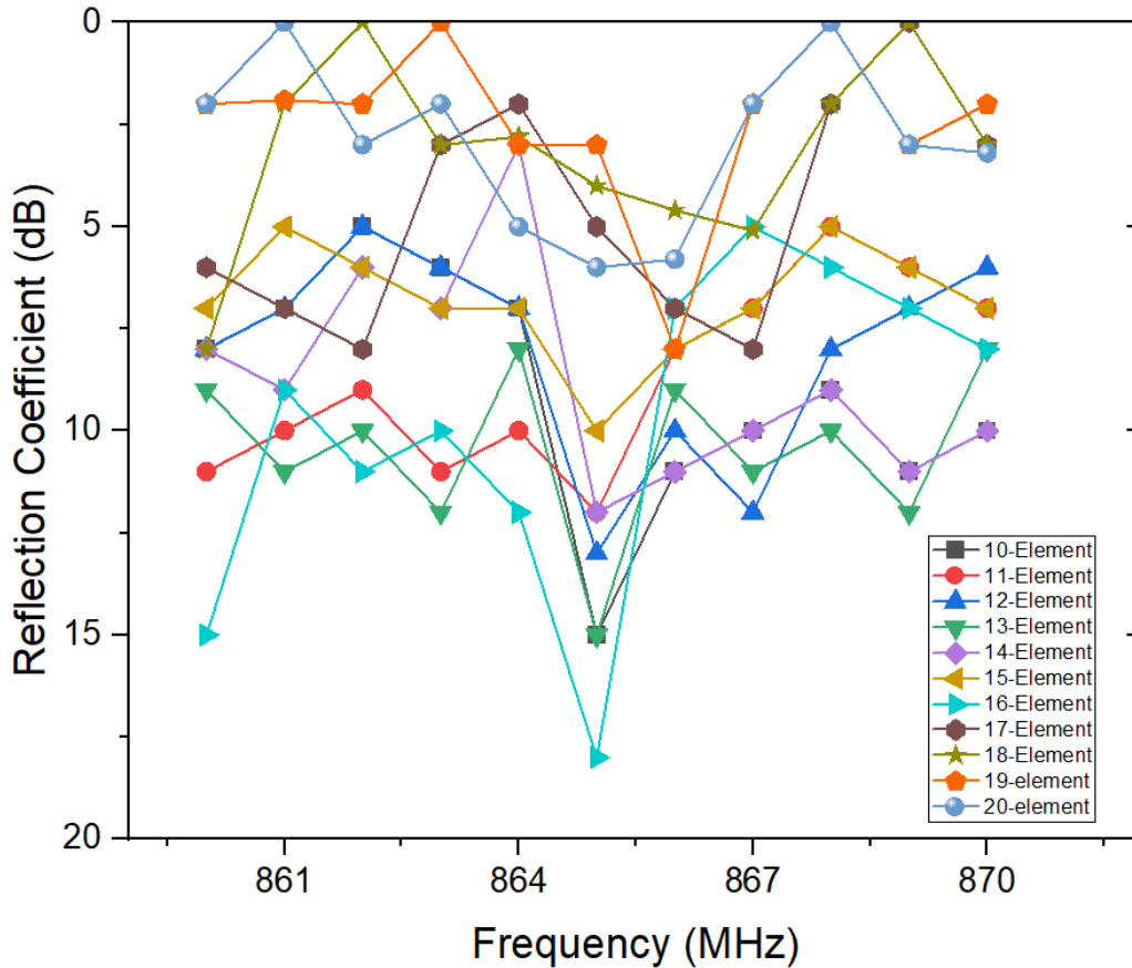
Fig. 4. Reflection coefficient for various elements of Bicone strip antenna at 865MHz
