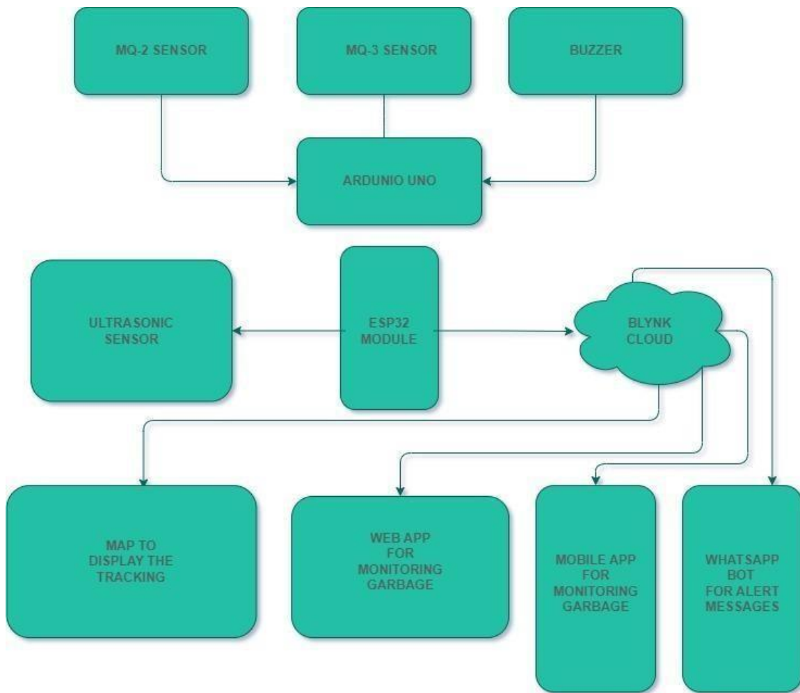
Figure 5.2: System Flowchart
