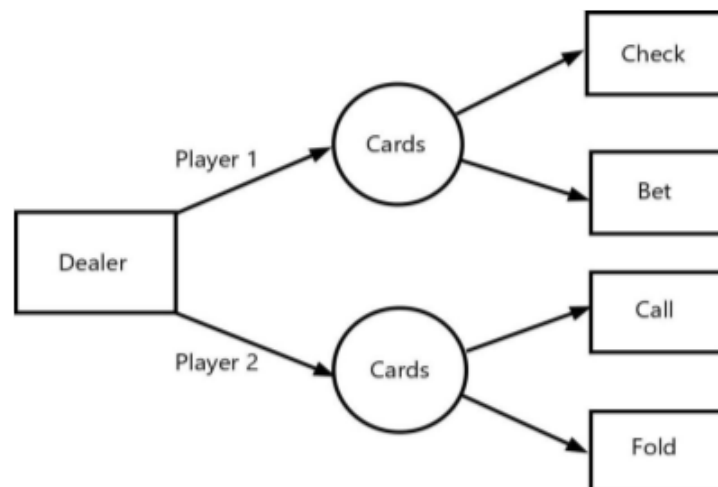
Figure 3.14 Von Neumann's Poker: Rule
