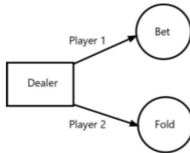
Figure 3.10 Borel Poker: Round 1: Case 2
