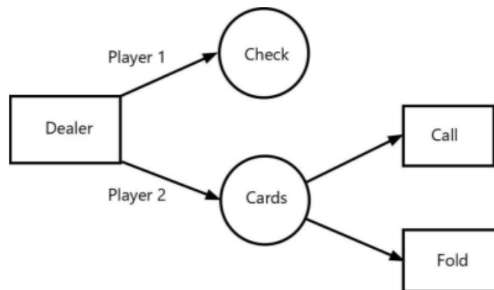
Figure 3.31 AKQ Game: Round 1
