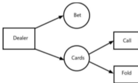
Figure 3.8 Borel Poker: Round 1
