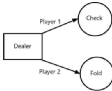
Figure 3.18 Von Neumann's Poker: Round 2: Case 2
