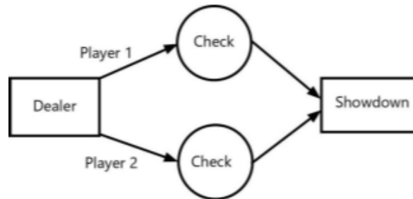
Figure 3.28 Clairvoyance Game: Case 1
