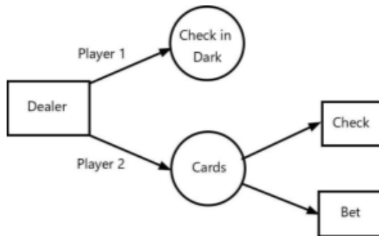
Figure 3.22 Half Street Games
