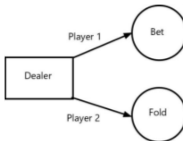
Figure 3.6 Uniform Poker Model: Round 2: Case 2
