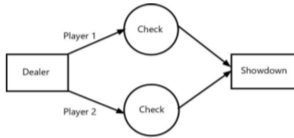
Figure 3.15 Von Neumann's Poker: Round 1
