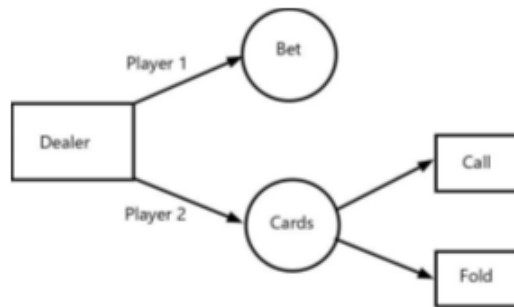
Figure 3.19 Von Neumann's Poker: Round 3
