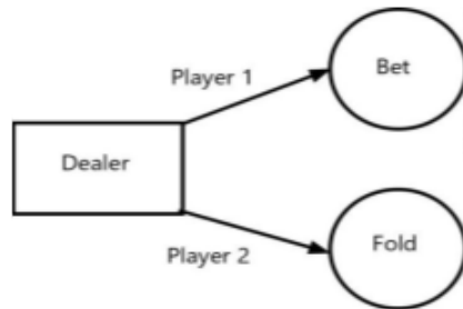
Figure 3.21 Von Neumann's Poker: Round 3: Case 2
