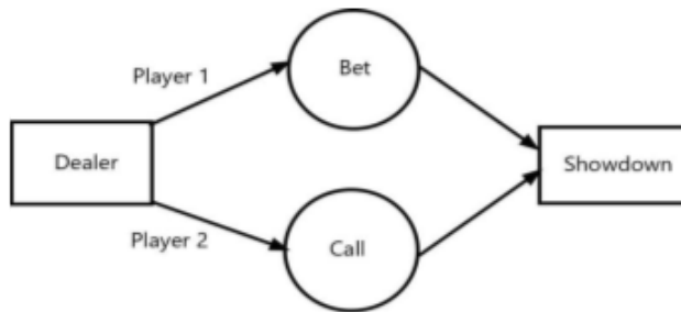
Figure 3.6 Uniform Poker Model: Round 2: Case 1
