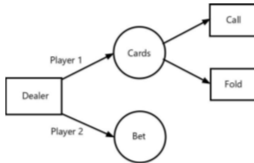
Figure 3.24 Half Street Games: Round 2
