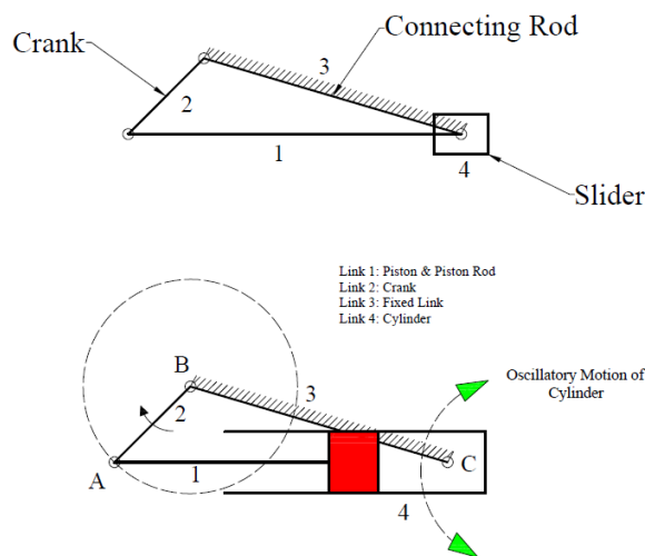
Figure: 11 Third Inversion (Oscillating Cylinder Engine Mechanism)
