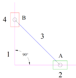
Figure: 14 2R-2P Mechanism
