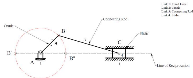
Figure: 9 First Inversion (Slider Crank Mechanism)
