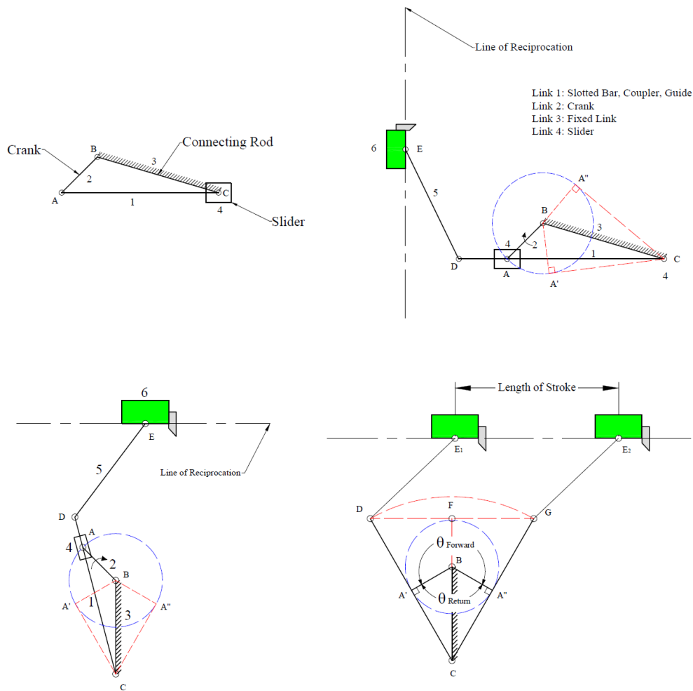
Figure: 12 Third Inversion (Crank & Slotted Lever Mechanism)
