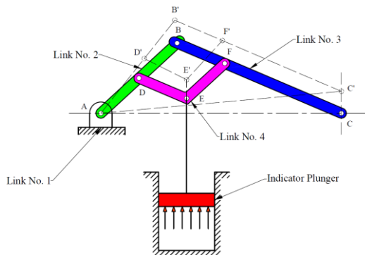
Figure: 22 Watt's Indicator Mechanism
