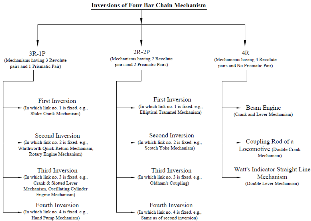
Figure: 8 Inversions of Four Bar Chain Mechanism
