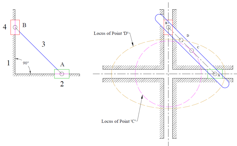
Figure: 15 First Inversion of 2R-2P (Elliptical Trammel)
