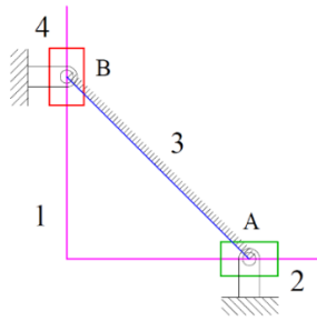
Figure: 18 Third Inversion of 2R-2P
