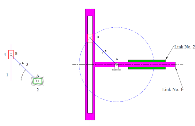
Figure: 17 Second Inversion of 2R-2P (Scotch Yoke Mechanism)
