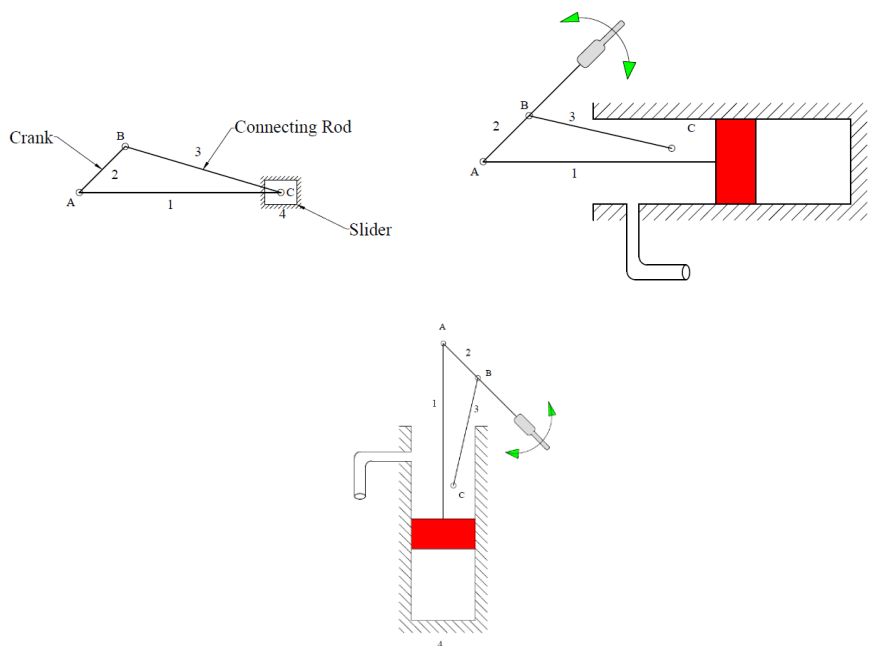
Figure: 13 Fourth Inversion (Hand Pump Mechanism)
