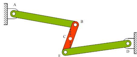
Figure: 23 Straight Line Mechanism
