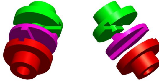
Figure: 19 Third Inversion of 2R-2P (Oldham's Coupling)
