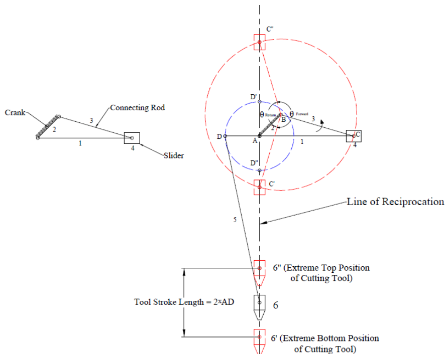
Figure: 10 Second Inversion (Whithworth Quick Return Mechanism)
