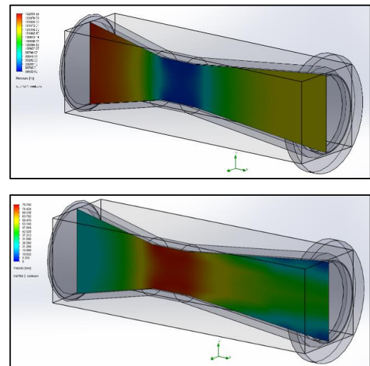
Figure 4: Pressure & Velocity Simulation (14°)
