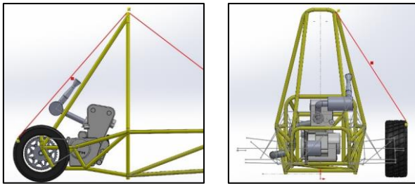
Figure 13: Side & Rear-View Surface Envelope
