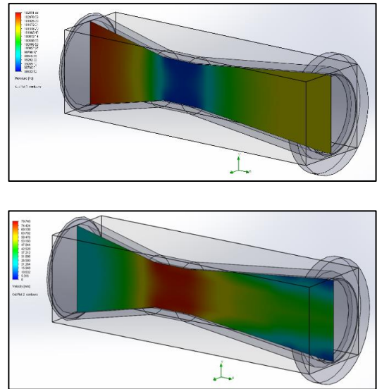
Figure 3: Pressure & Velocity Simulation (12°)
