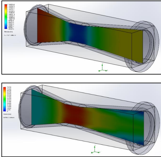
Figure 5: Pressure & Velocity Simulation (16°)
