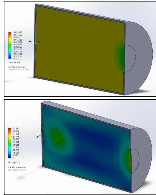
Figure 11: Pressure & Velocity Simulation (Cylindrical)
