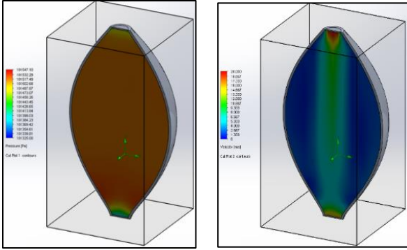
Figure 8: Pressure & Velocity Simulation (Elliptical)
