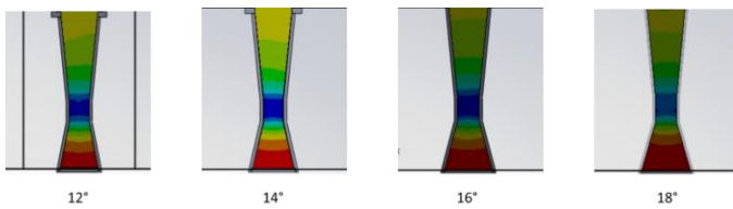
Figure 2: Venturi with different Converging angle
