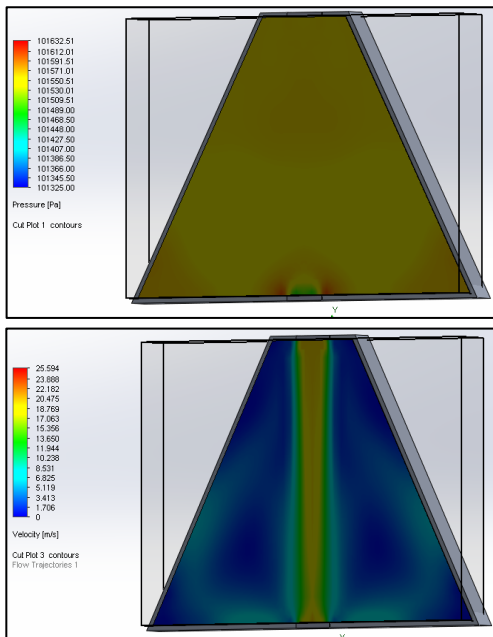
Figure 9: Pressure & Velocity Simulation (Triangular)
