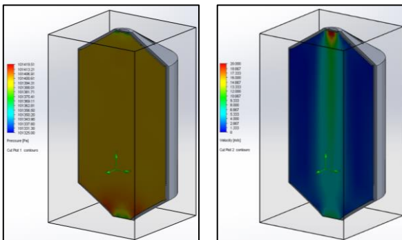
Figure 10: Pressure & Velocity Simulation (Conical)
