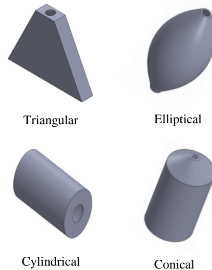
Figure 7: Intake Plenum CAD Models
