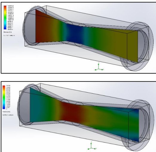
Figure 6: Pressure & Velocity Simulation (18°)
