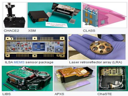
Fig 12: Pragyan rover instruments
