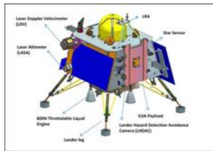
Fig 17: Lander
