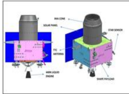
Fig 16: Propulsion module
