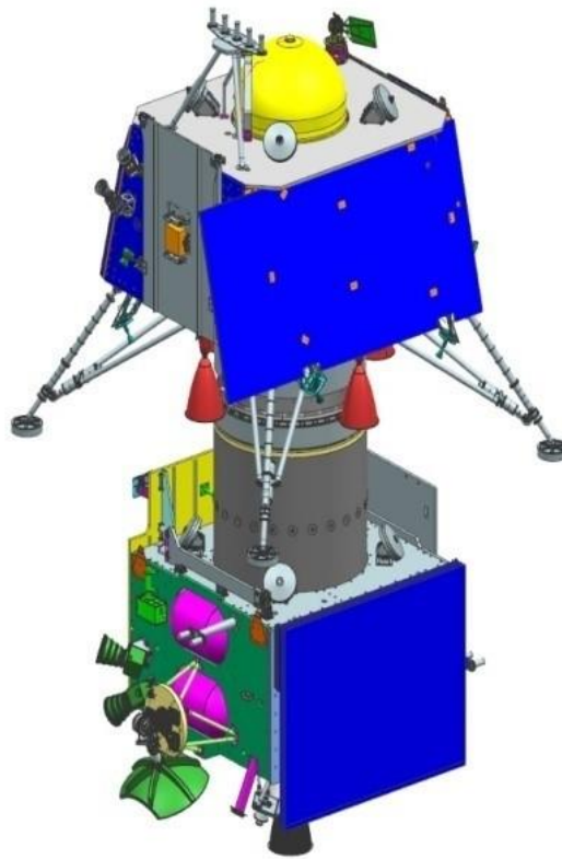
Fig 9: Chandrayaan 2 composite
