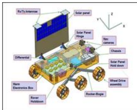
Fig 18: Pragyna Rover
