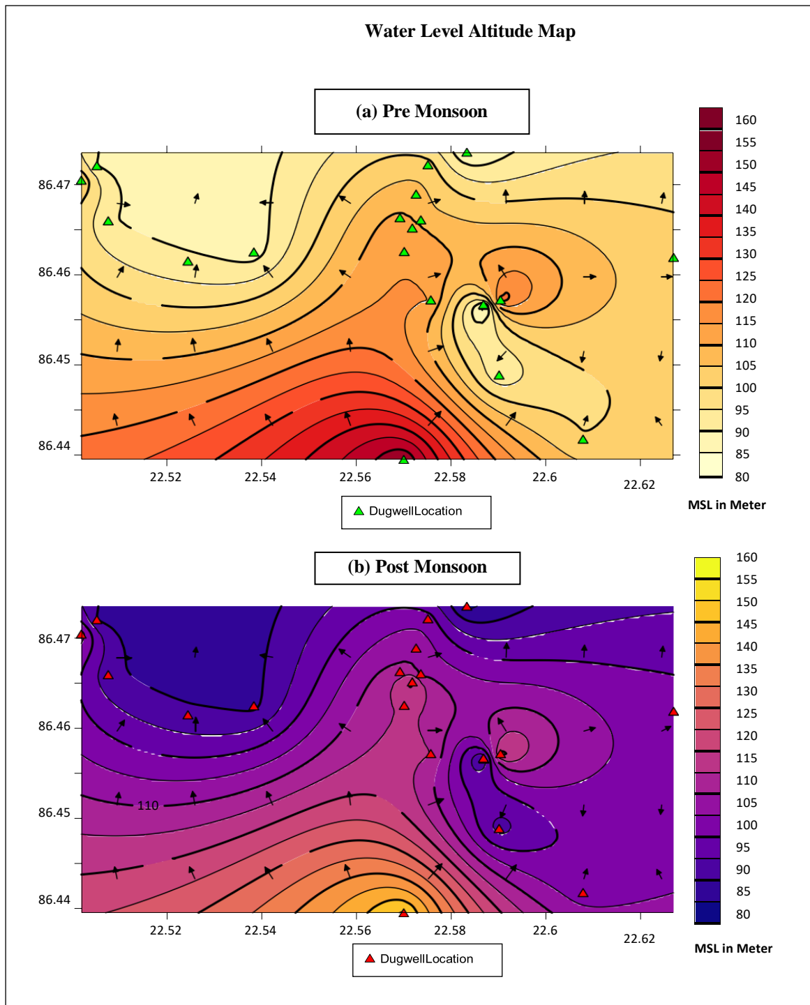
Fig. 3: Groundwater Contour Map of Study Area showing dominant flow directions
