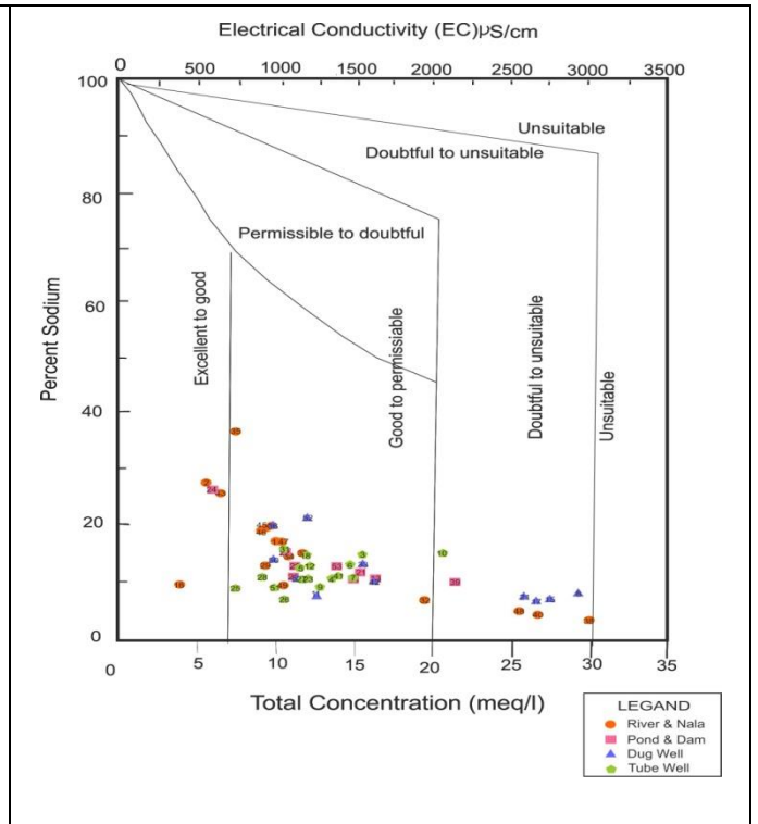
Fig.6. Classification of Groundwater Quality for Irrigation (after Wilcox, 1954).
