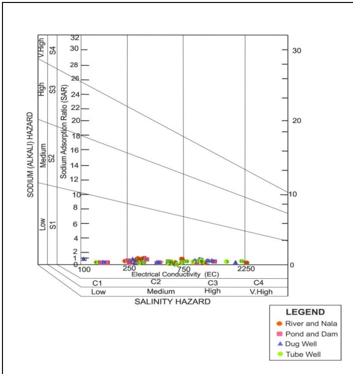
Fig.5. Classification of Groundwater Quality for Irrigation (after Richards, 1954).
