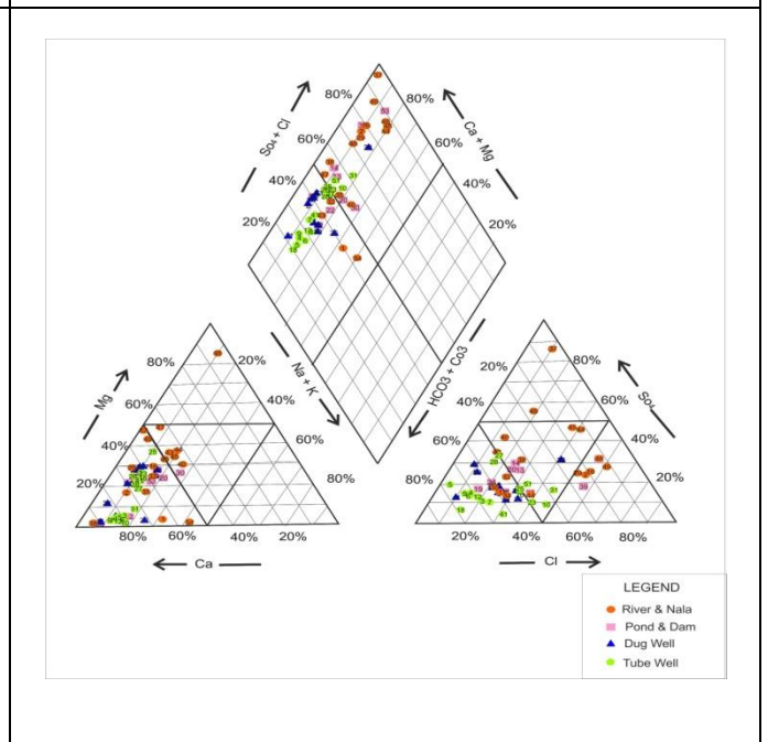
Fig.8. Classification of Groundwater Quality for Irrigation (after Piper, 1944).
