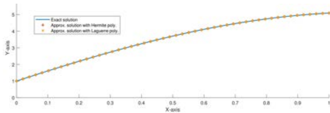
Figure 4. Graph of exact and approximate solution of case 2 with Hermite and Laguerre polynomials (n=6)
